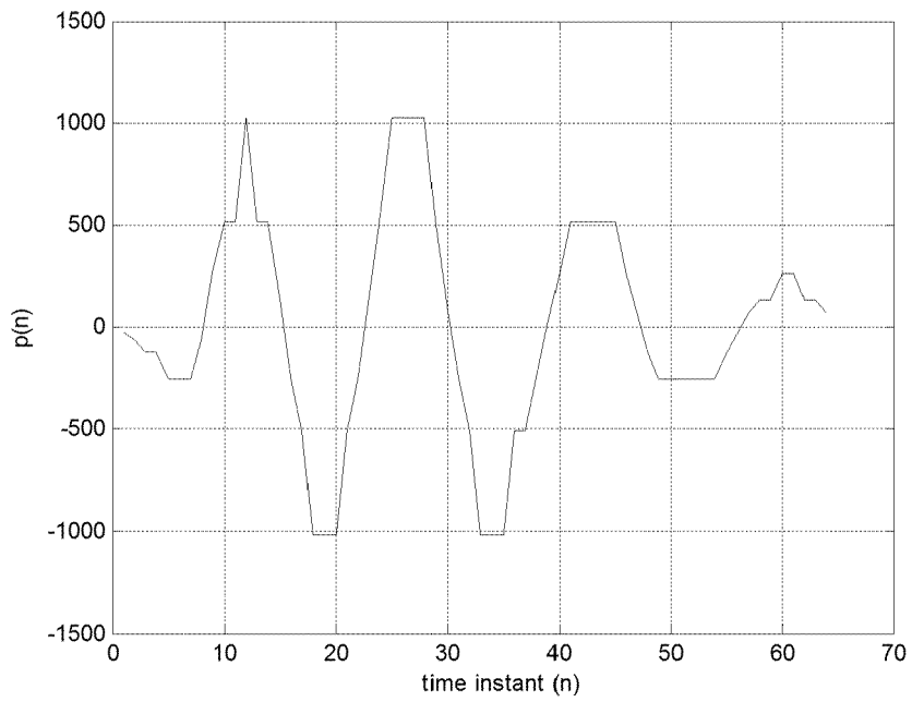
Figure 4b: Match filter corresponding to the pulse in Figure 1
