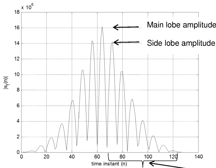
Figure 4c: Absolute value of the match filtered ultrasound signal. The upper arrow indicates the amplitude of the main lobe, the middle arrow indicates the amplitude of the largest side lobe and the lower arrow indicates "all" the side lobes that are considered for some of the selection criteria.
