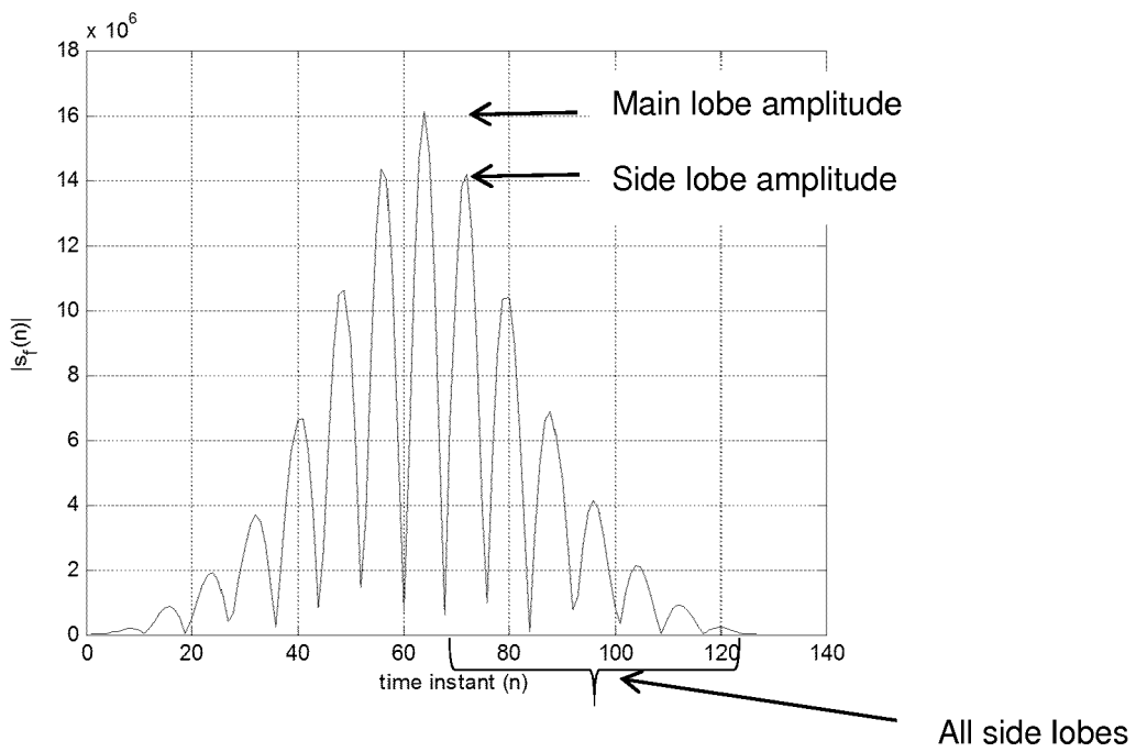
Figure 4c: Absolute value of the match filtered ultrasound signal. The upper arrow indicates the amplitude of the main lobe, the middle arrow indicates the amplitude of the largest side lobe and the lower arrow indicates “all” the side lobes that are considered for some of the selection criteria.
