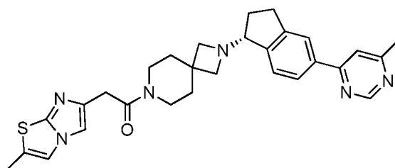
(R)-2-(2-methylimidazo[2,1-b]thiazol-6-yl)-1-(2-(5-(6-methylpyrimidin-4-yl)-2,3-dihydro-1H-inden-1-yl)-2,7-diaza-spiro[3.5]nonan-7-yl)ethanone
