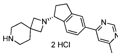
2-[(R)-5-(6-methyl-pyrimidin-4-yl)-indan-1-yl]-2,7-diaza-spiro[3.5]nonane dihydrochloride
