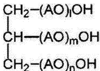
Structural Formula (1)
