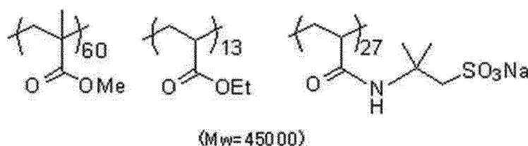
Water-soluble polymer 1
