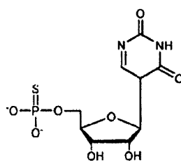
5'-O-(1-Thiophosphate)-Pseudouridine
