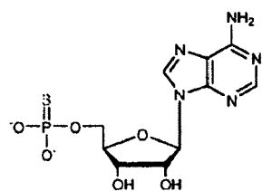
5'-O-(1-Thiophosphate)-Adenosine
