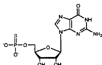
5'-O-(1-Thiophosphate)-Guanosine
