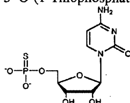
5'-O-(1-Thiophosphate)-Cytidine
