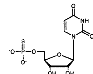
5'-O-(1-Thiophosphate)-Uridine
