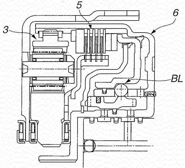
FIG.13B HYDRAULIC PRESSURE OFF
