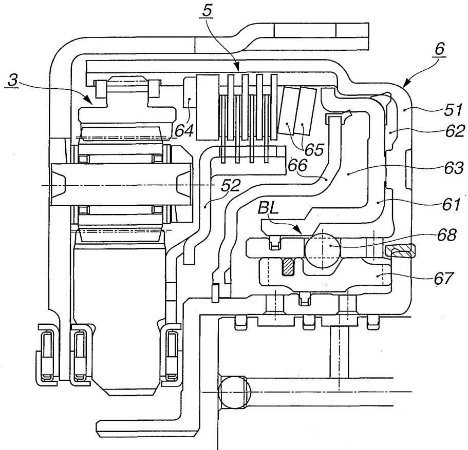
FIG.12A STATE CHANGE (CLUTCH OPEN)
