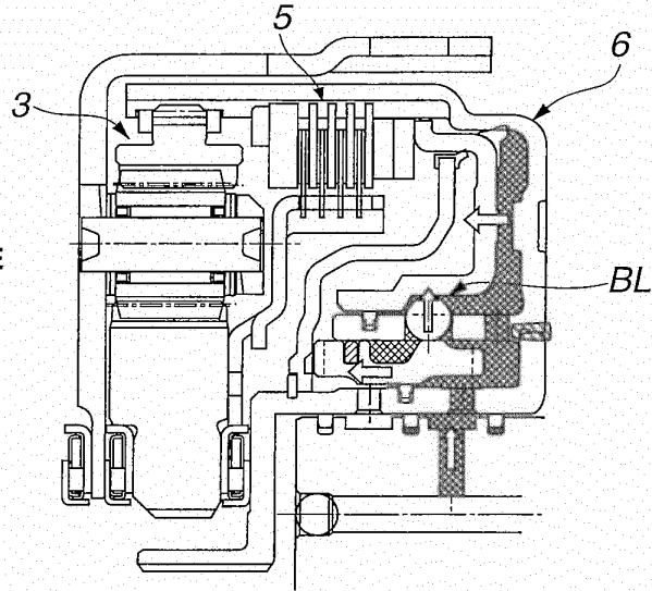
FIG.13A FWD/C ON PRESSURE CHARGE
