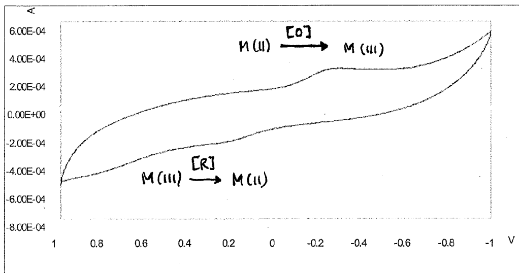
Current (A) vs. Potential (V) vs. Ag/AgCl Reference Electrode
