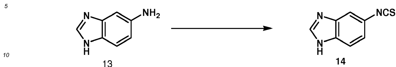
Scheme 4: Synthesis of 5-isothiocyanato-1H-benzo[d]imidazole (14)
