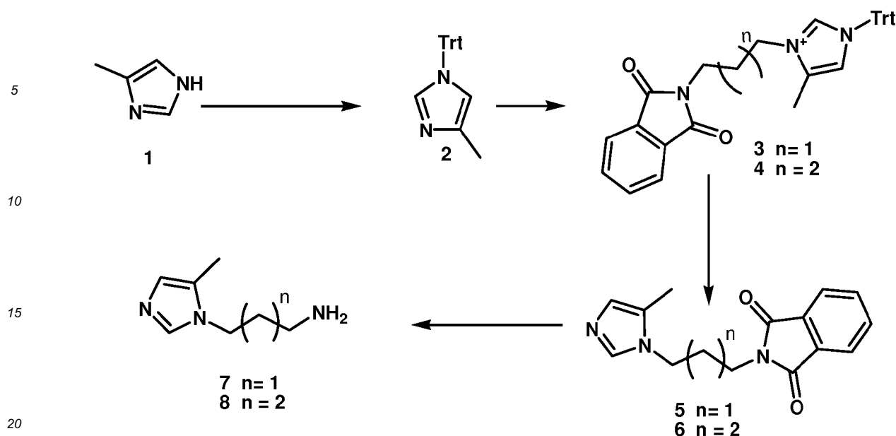
Scheme 2: Synthesis of the 3-(5-methyl-1H-imidazol-1-yl)alkyl-1-amines (7 and 8)
