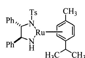
Catalyst c
