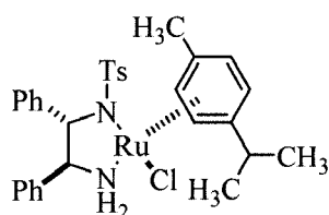
Catalyst a
