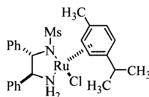
Catalyst b
