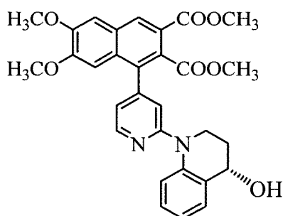
[d-11]
