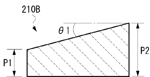
(B) Enlarged sectional view taken along line B1-B1
