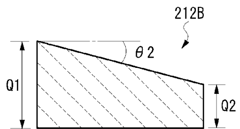
(C) Enlarged sectional view taken along line B2-B2
