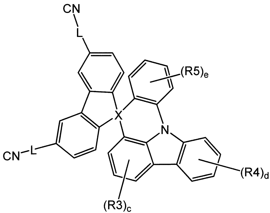
[Chemical Formula 1-4]
