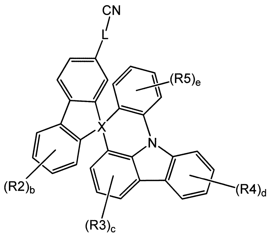
[Chemical Formula 1-2]
