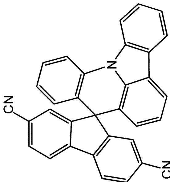
Chemical Formula 2-3
