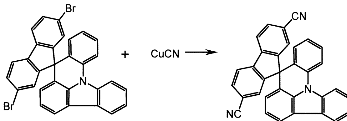
[Compound A]
