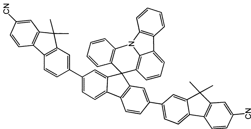
Chemical Formula 2-17
