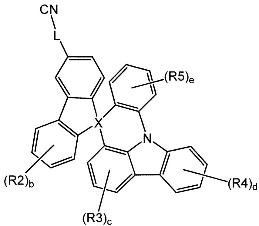
[Chemical Formula 1-2]
