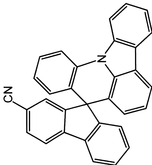
Chemical Formula 2-1
