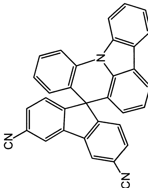
Chemical Formula 2-4
