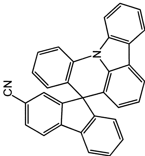
Chemical Formula 2-1
