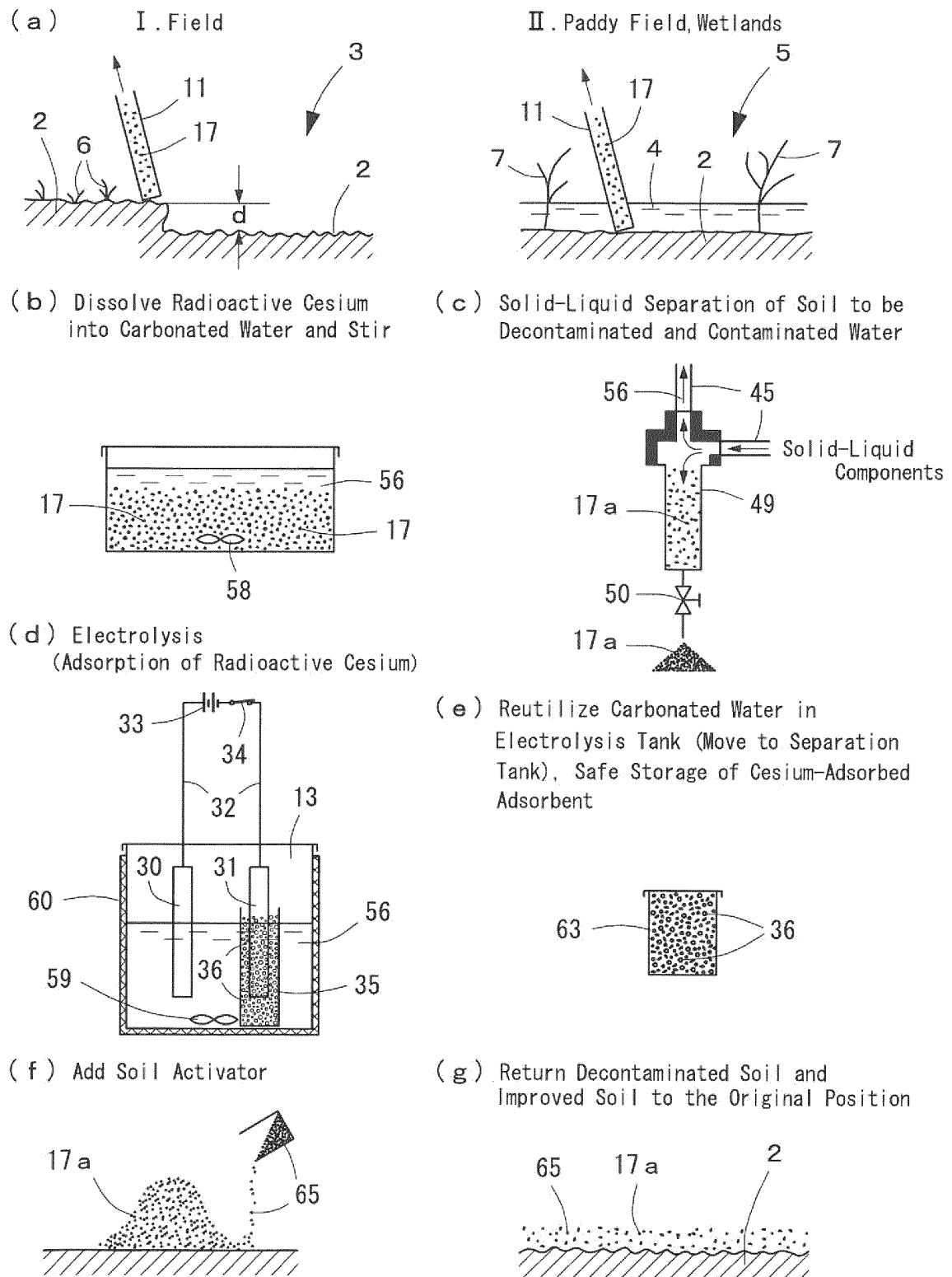
Fig. 4 Procedure of Decontamination Work for Soil of the Present Invention
