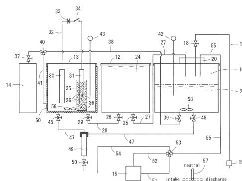
Fig. 5 Before Introduction of Contaminated Soil and Before Separation of Cesium
