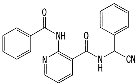
[Chem. 1]
