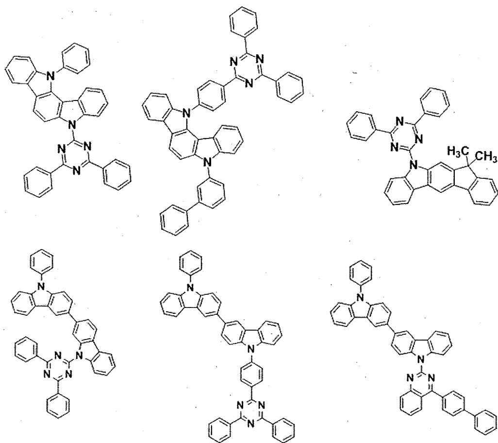
[Chemical Formula 27]
