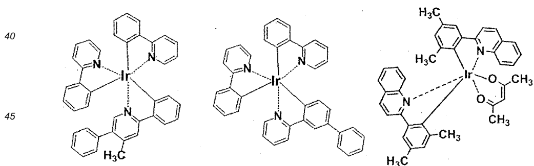
[Chemical Formula 29]
