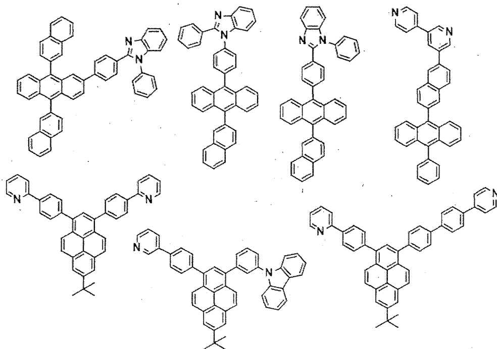
[Chemical Formula 30]
