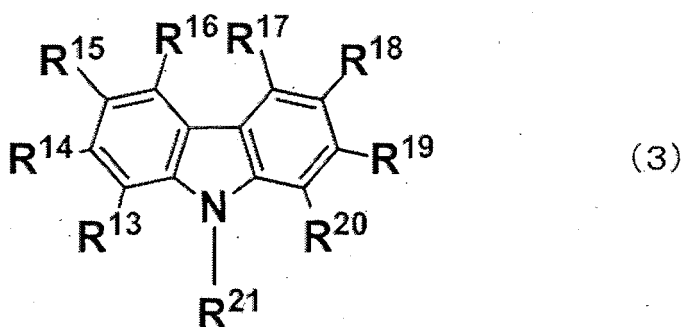
[Chemical Formula 6]
