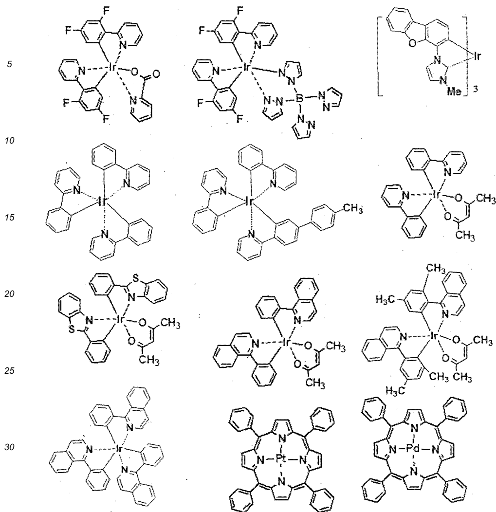
[Chemical Formula 29]
