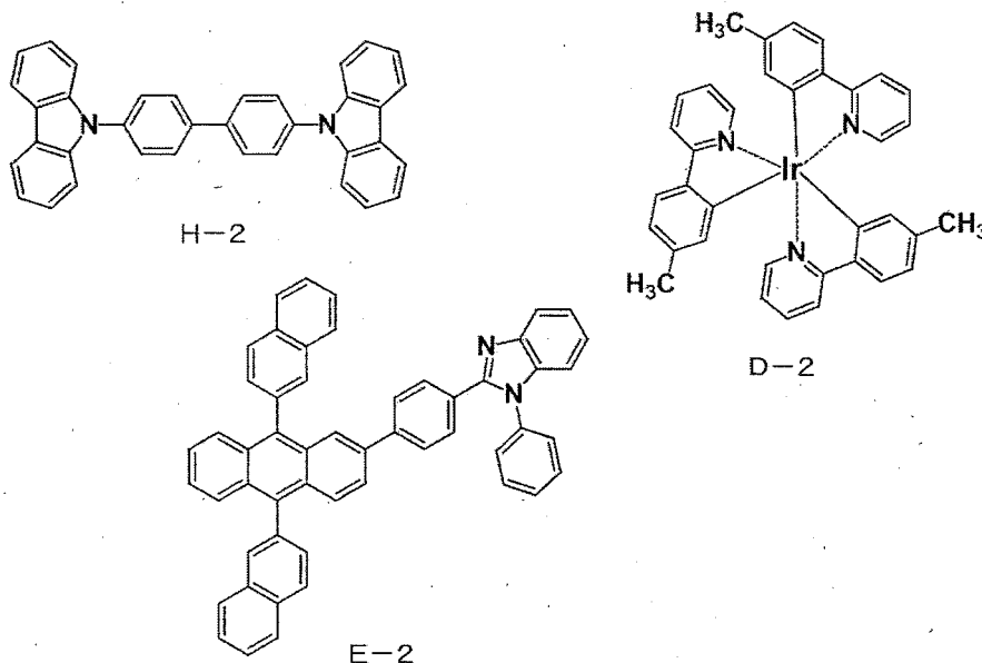
[Chemical Formula 34]
