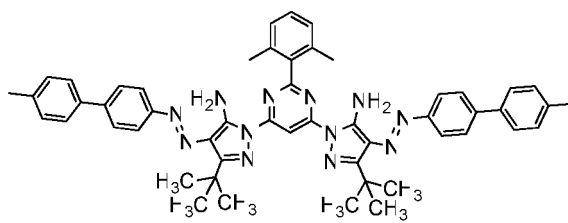
Compound (33)
