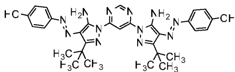
Compound (34)
