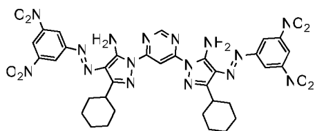
Compound (32)
