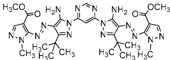
Comparative compound (1)
