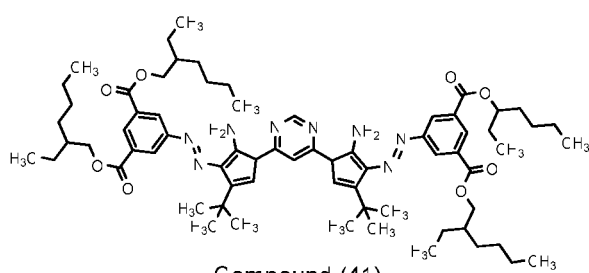
Compound (41)
