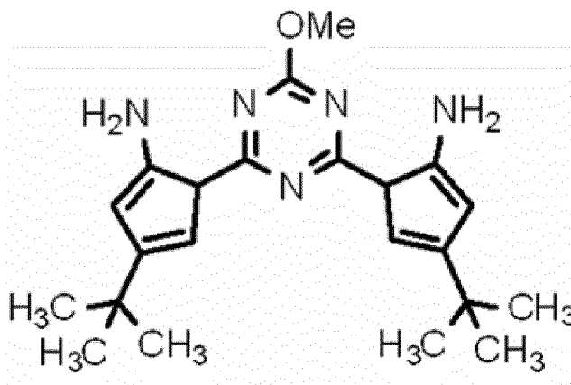
Triazine compound (1)
