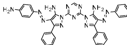
Compound (35)
