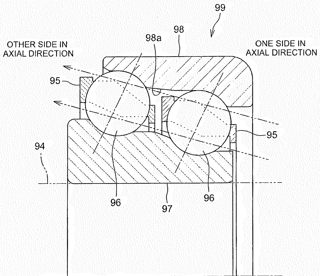
FIG. 8 RELATED ART
