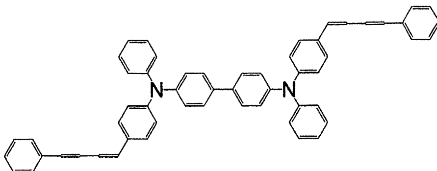
[Chem. 49]
