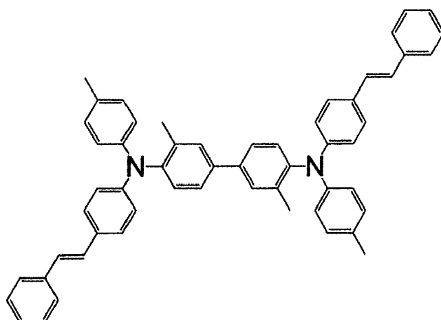
[Chem. 48]
