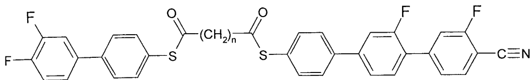
F-GIP-SConCOS-PGG-N
