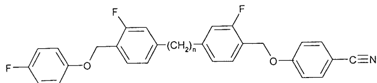
F-PO1GI-n-GO1P-N (= N-PO1GI-n-GO1P-F)
