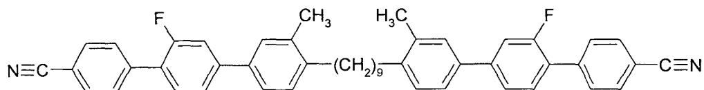
N-PGIP(1)-9-PI(1)GP-N
