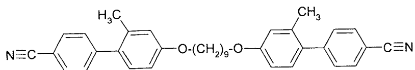
N-PPI(1)-O9O-P(1)P-N
