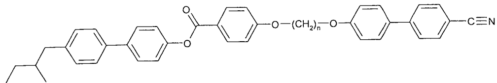
2(CHCH3)1-PPZIP-OnO-PP-N
