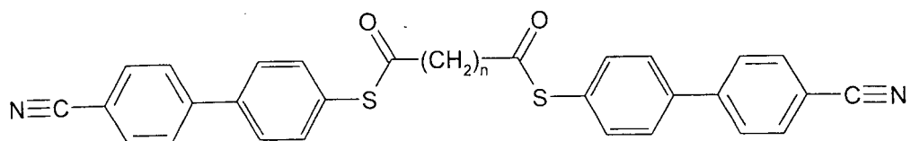
N-PP-SConCOS-PP-N
