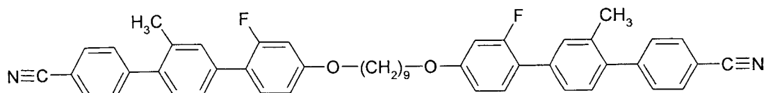
N-PPI(1)P-O9O-PP(1)P-N
