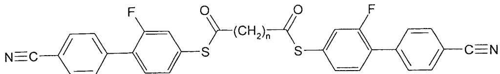
N-PGI-SConCOS-GP-N
