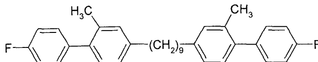
F-PPI(1)-9-(1)PP-F
