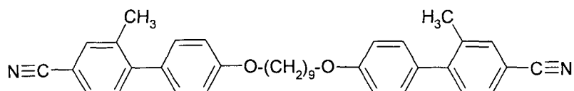
N-P(1)P-O9O-PPI(1)-N
