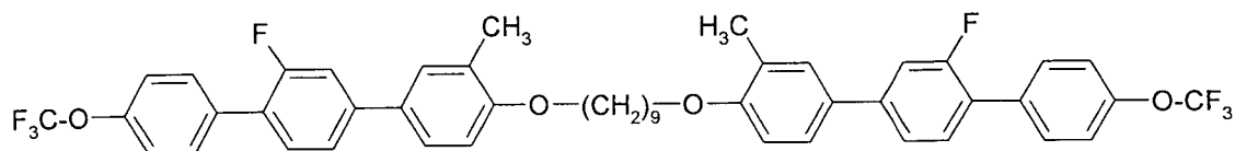
N-PGIP(1)-O9O-PI(1)GP-N
