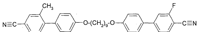
N-P(1)P-O9O-PG-N
