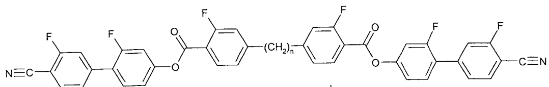
N-GIGIZIGI-n-GZGG-N
