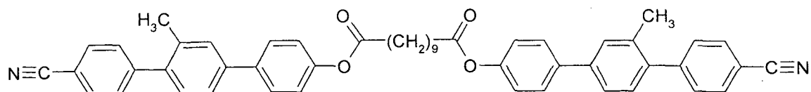
N-PPI(1)P-ZI9Z-PP(1)P-N
