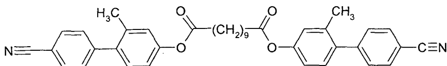
N-PPI(1)-ZI9Z-P(1)P-N
