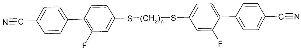
N-PP-SnS-PP-N
