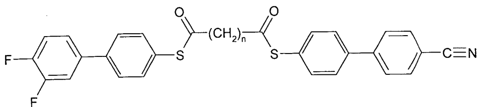
F-GIP-SConCOS-PP-N
