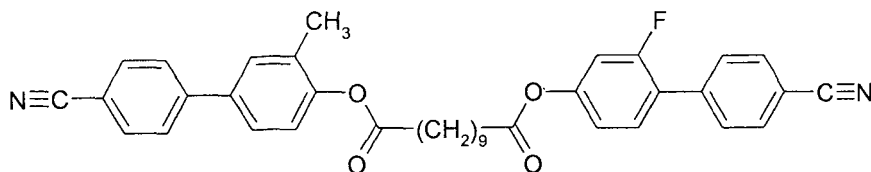
N-PP(1)-ZI9Z-PG-N
