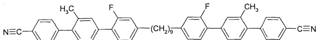
N-PPI(1)GI-ZI9Z-GP(1)P-N
