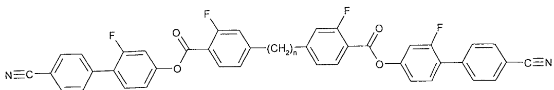
N-PGIZIGI-n-GZGP-N
