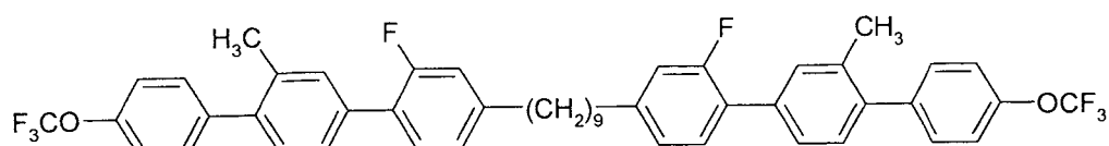
TO-PPI(1)GI-9-GP(1)P-OT
