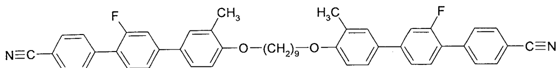
N-PGIP(1)-O9O-PI(1)GP-N
