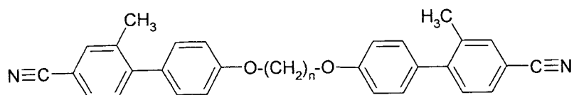
N-P(1)P-OnO-PPI(1)-N
