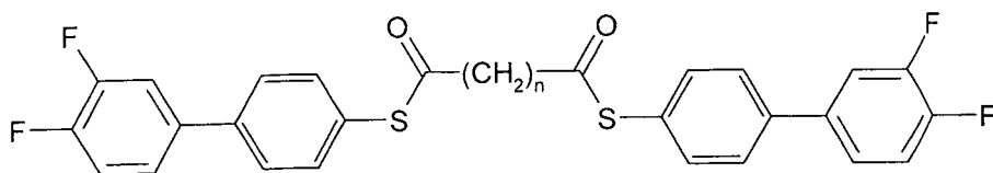
F-GIP-SConCOS-PG-F
