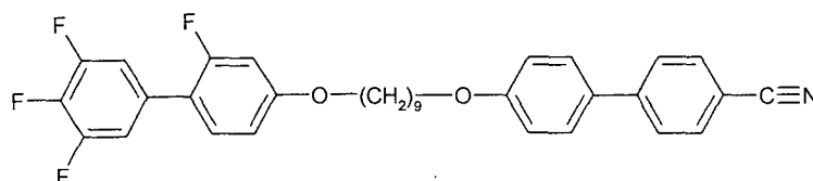
F-UIGI-O9O-PP-N
