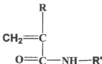
[Chemical Formula 4]
