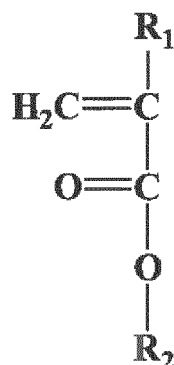
[Chemical Formula 4]
