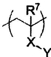
Formula (4)
