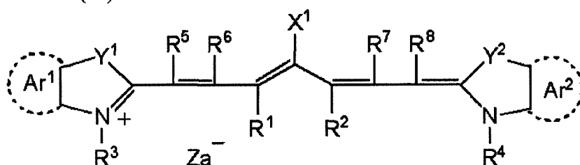
Formula (IV)
