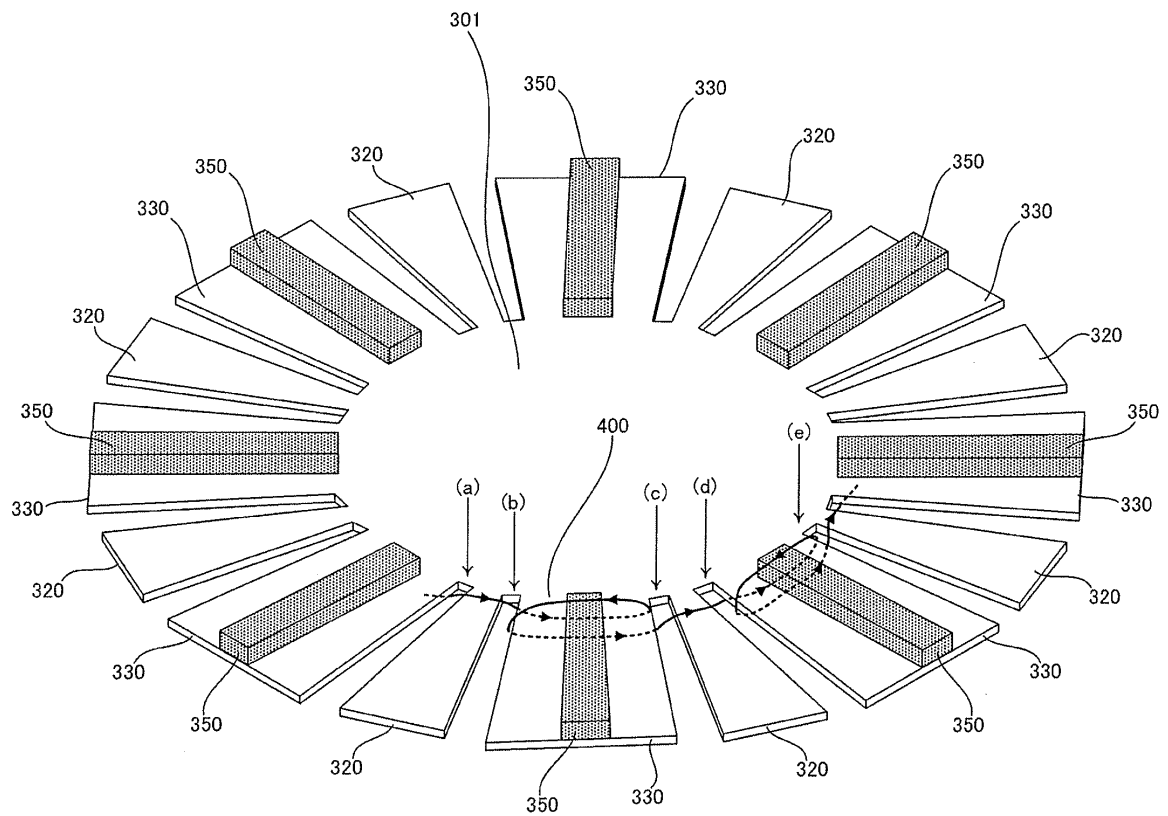
Diagram illustrating winding pattern of conductive line 400
