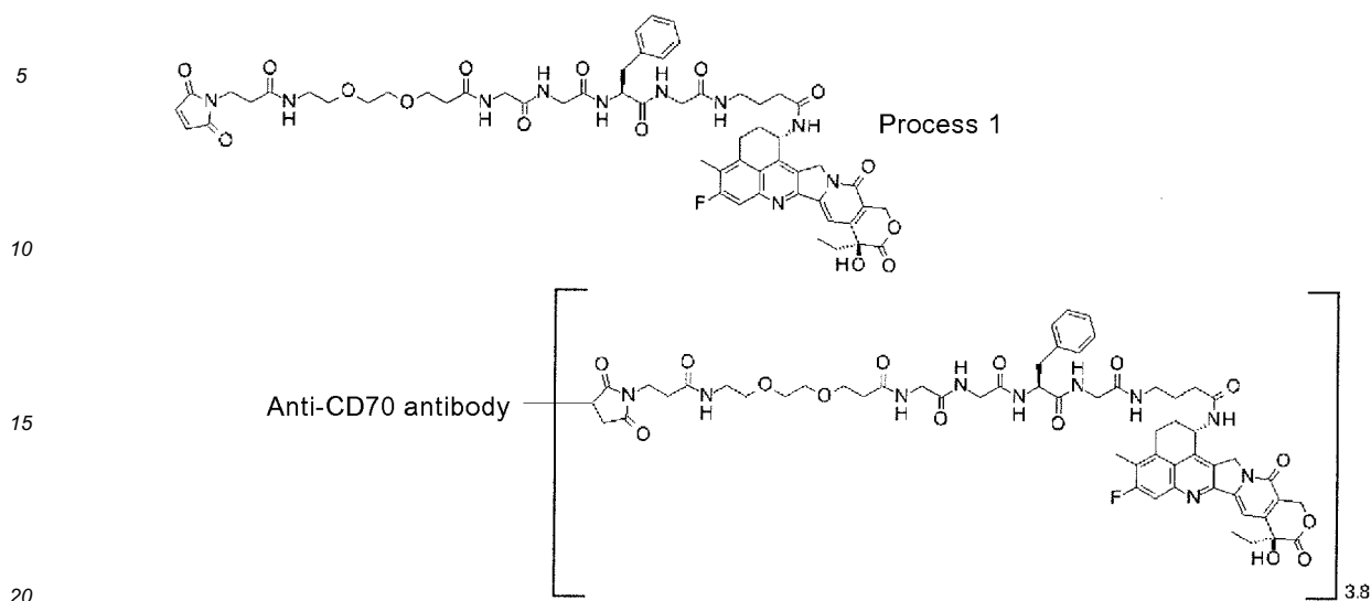
Process 1: Antibody-drug conjugate (26)
