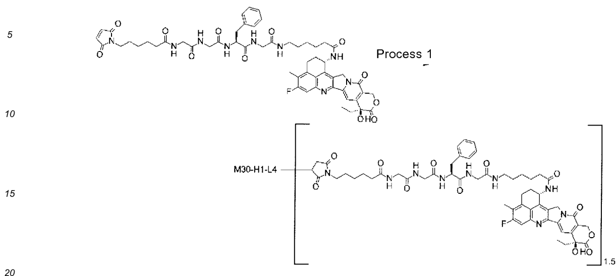
Process 1: Antibody-drug conjugate (53)
