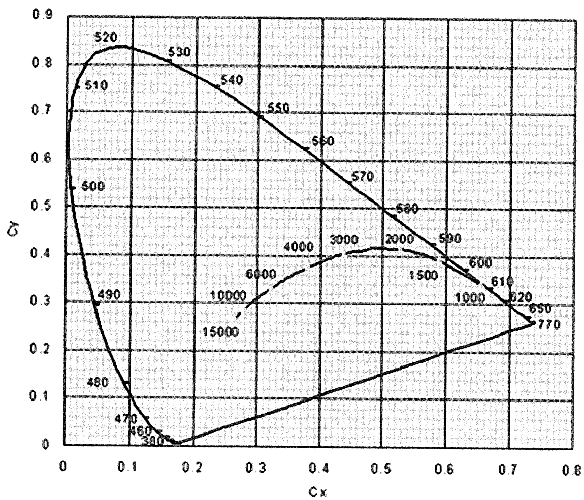
CIE1931 Chromaticity Diagram
