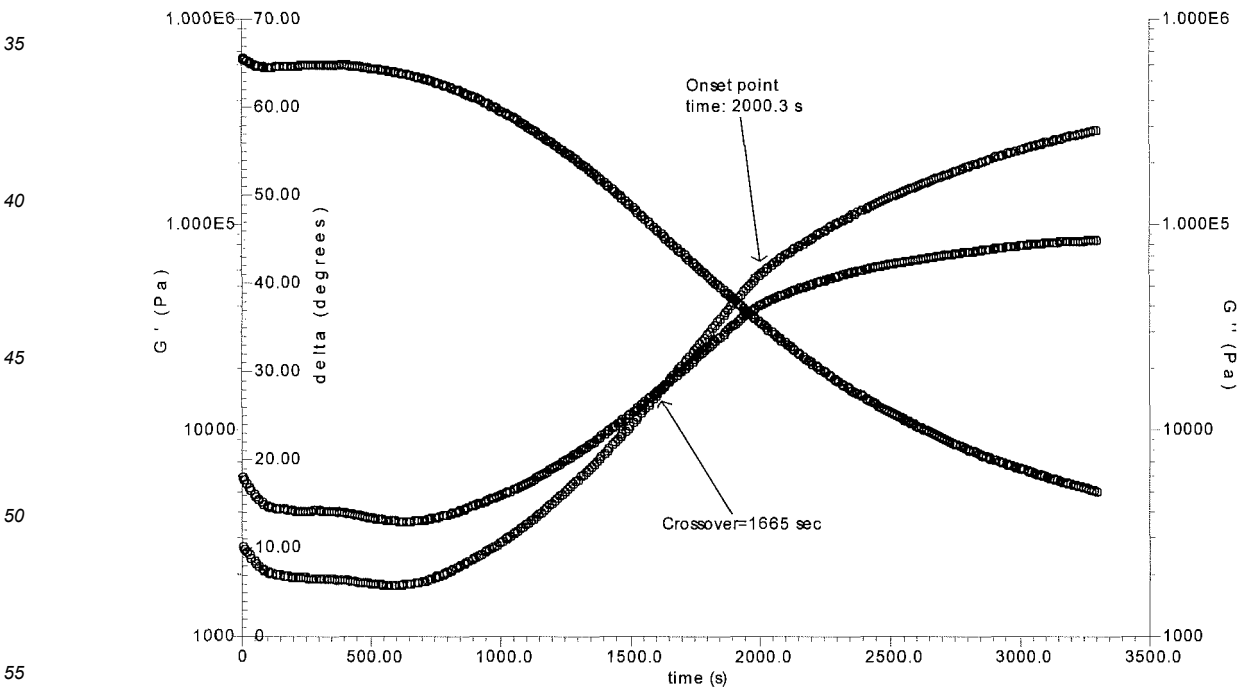
Graph 1. Parallel Plate Rheology of Blend 3, at 380 °C. See, J. Mercel et al., "Thermal Analysis of Polymers: Fundamentals and Applications," p. 445, Wiley, ed. 1 (2009).
