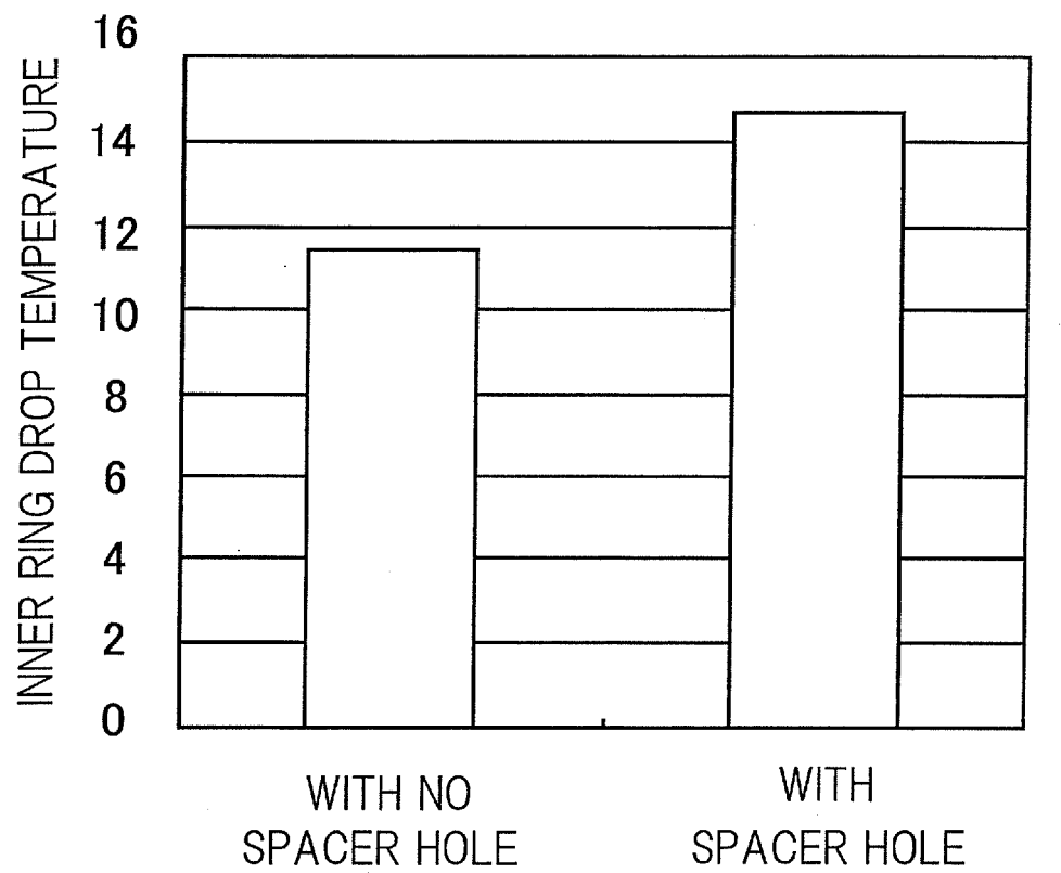
COMPARISON OF INNER RING DROP TEMPERATURE
