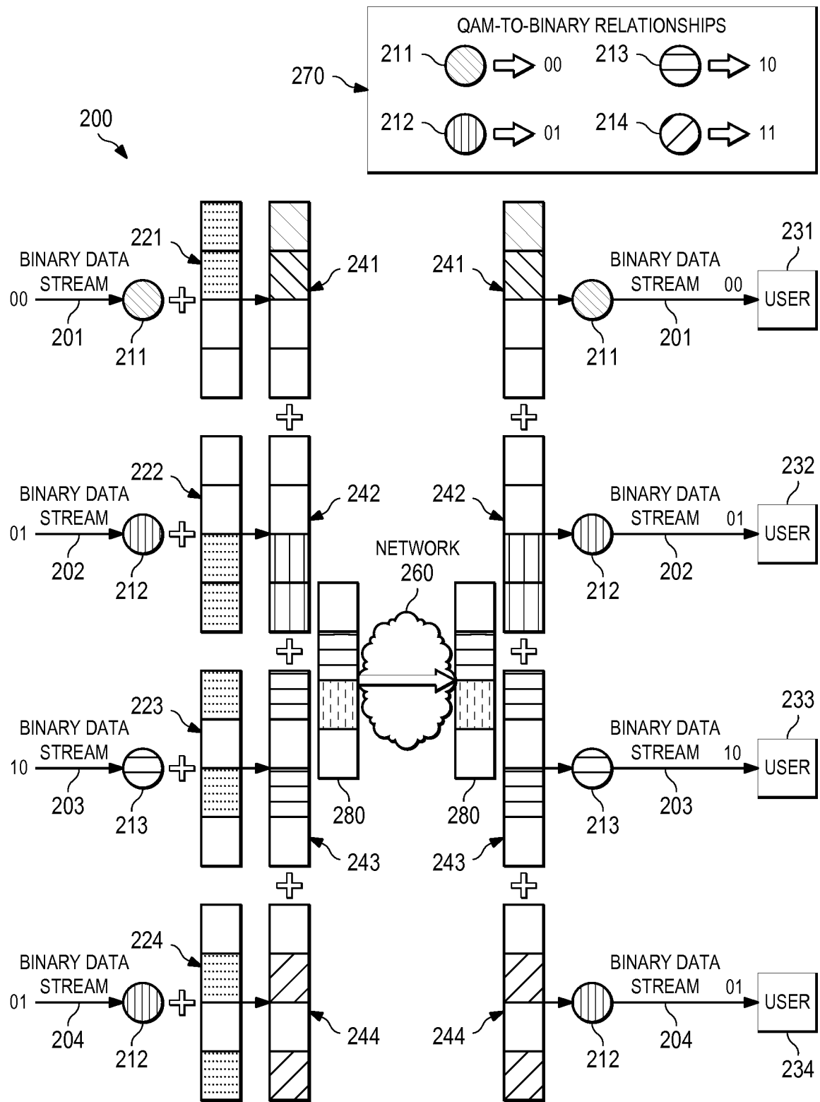
FIG. 2 (PRIOR ART)
