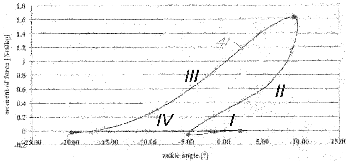
Moment of force vs. ankle angle
