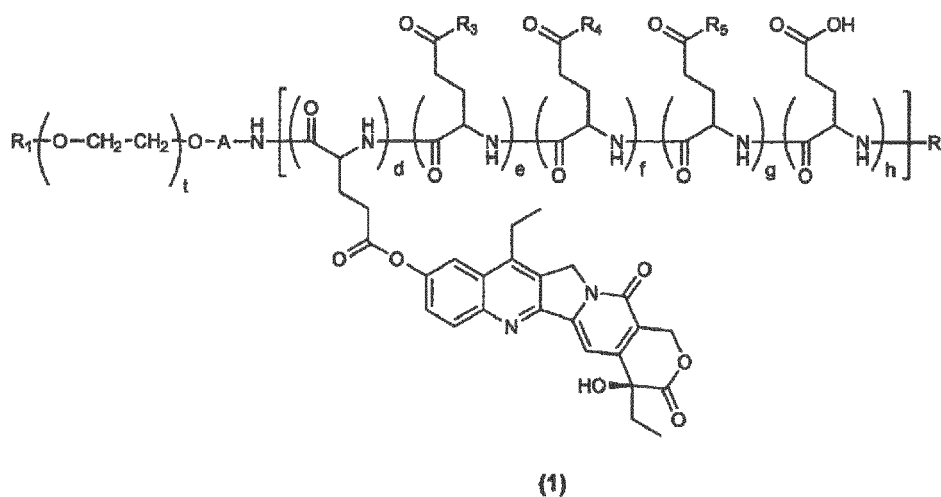
[Chemical Formula 1]
