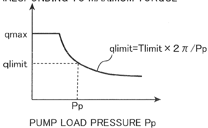
FIG. 9 PUMP DISPLACEMENT VOLUME CORRESPONDING TO MAXIMUM TORQUE
