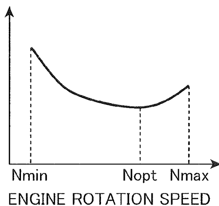
FIG. 8 ENGINE FUEL CONSUMPTION RATE
