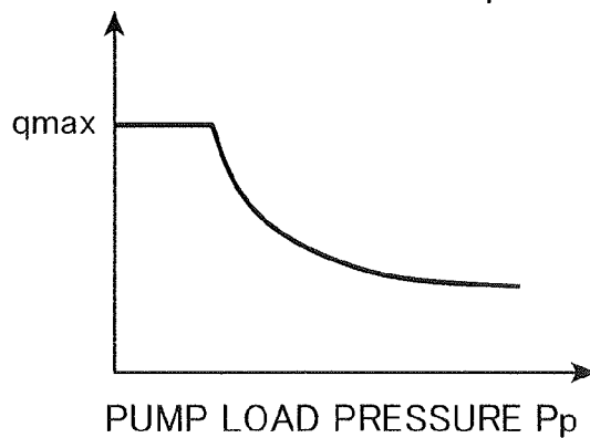
FIG. 7 TARGET PUMP DISPLACEMENT VOLUME FOR HORSEPOWER CONTROL q_h
