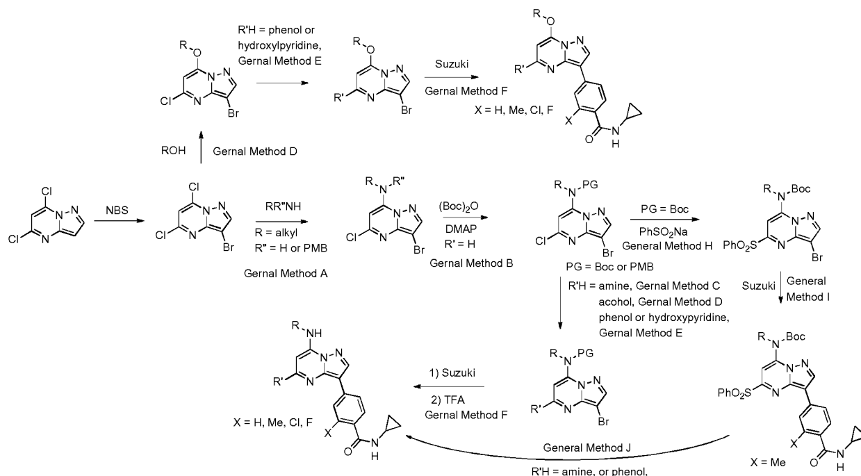
Scheme 4
