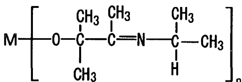
Compound No.15
