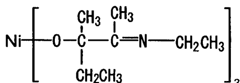
Compound No.44
