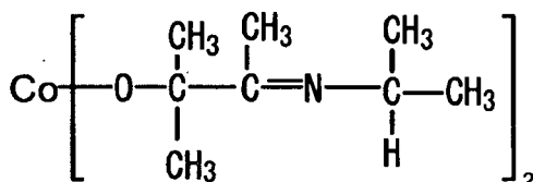
Compound No.63
