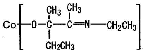
Compound No.60
