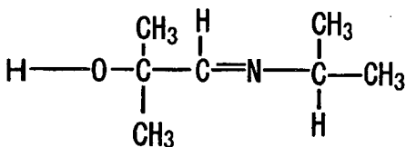
Compound No.71
