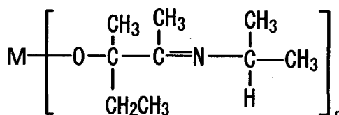
Compound No.16
