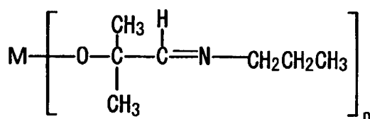
Compound No.5
