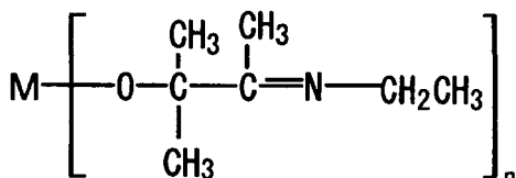
Compound No.11
