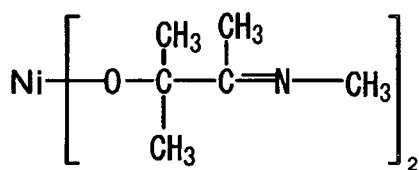
Compound No.41
