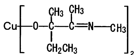
Compound No.26
