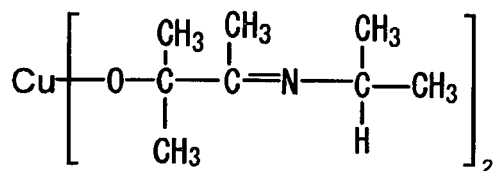
Compound No.31
