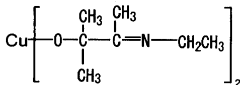
Compound No.27
