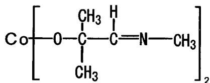
Compound No.49
