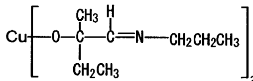
Compound No.22
