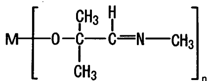
Compound No.1
