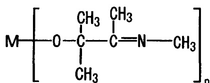
Compound No.9
