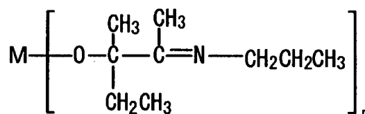
Compound No.14
