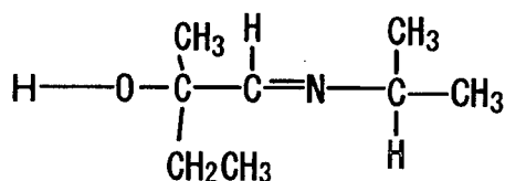
Compound No.72
