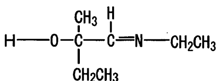
Compound No.68
