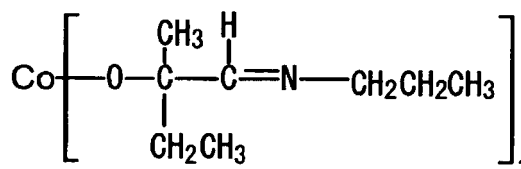
Compound No.54
