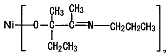
Compound No.46
