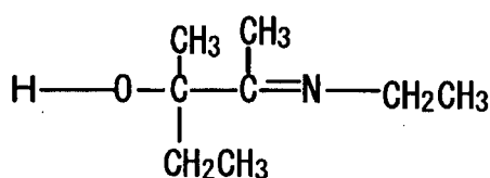
Compound No.76
