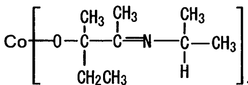
Compound No.64
