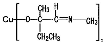
Compound No.18
