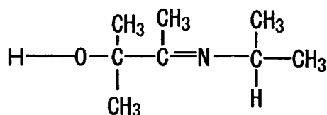
Compound No.74
