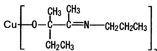
Compound No.30
