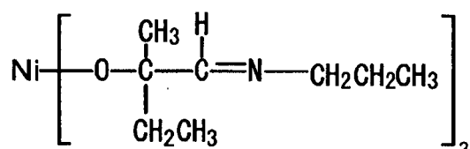
Compound No.38
