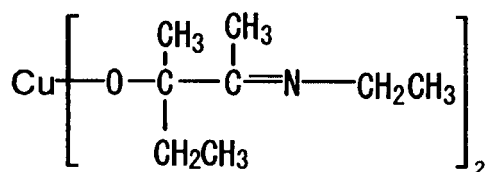
Compound No.28
