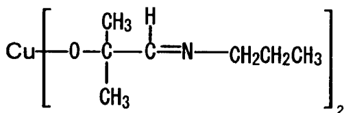
Compound No.21
