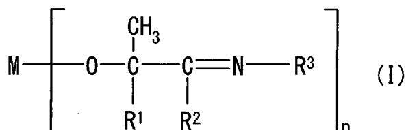
[Chem. 1]
