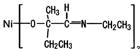
Compound No.36
