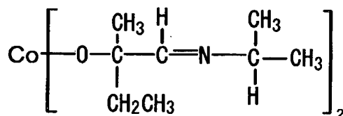
Compound No.56
