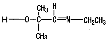
Compound No.67
