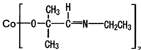
Compound No.51
