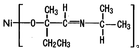
Compound No.40
