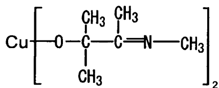
Compound No.25
