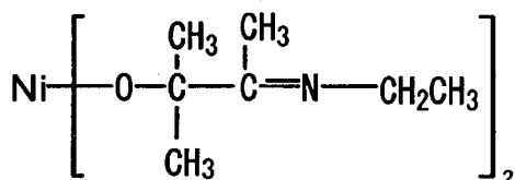
Compound No.43
