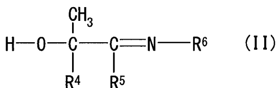
[Chem. 2]
