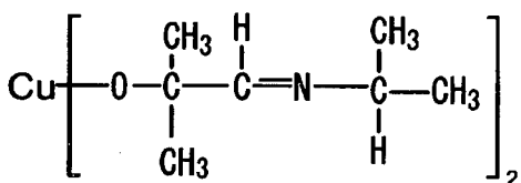
Compound No.23
