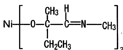
Compound No.34
