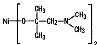
Comparative Compound 2
