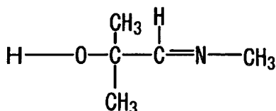
Compound No.65
