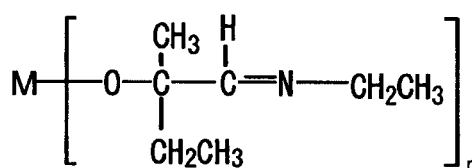
Compound No.4
