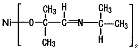
Compound No.39
