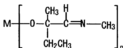
Compound No.2
