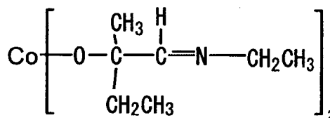
Compound No.52
