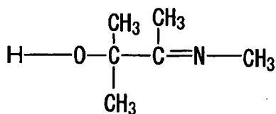
Alcohol Compound 1
