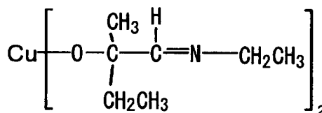
Compound No.20
