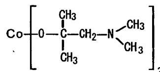
Comparative Compound 3
