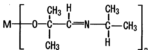
Compound No.7
