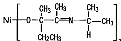
Compound No.48
