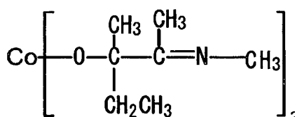
Compound No.58
