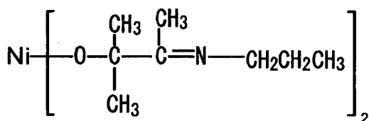
Compound No.45
