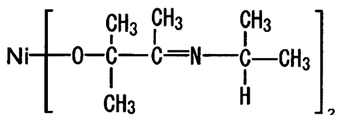
Compound No.47
