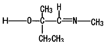
Compound No.66
