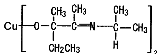
Compound No.32
