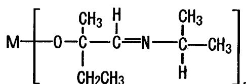
Compound No.8
