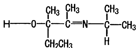
Compound No.78
