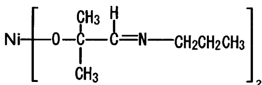
Compound No.37
