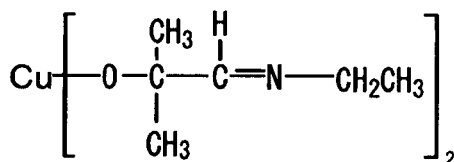
Compound No.19
