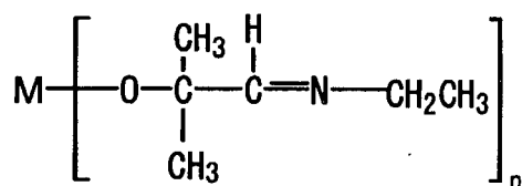
Compound No.3
