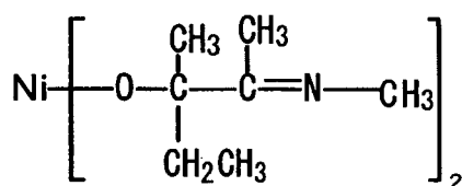
Compound No.42
