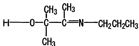
Compound No.73
