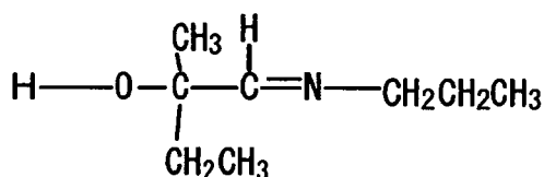
Compound No.70
