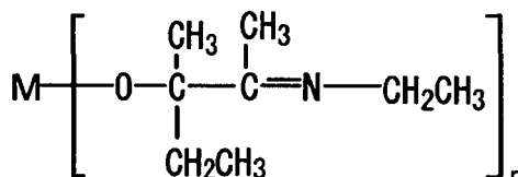
Compound No.12
