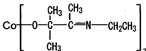
Compound No.59
