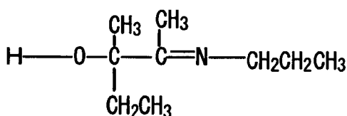
Compound No.77
