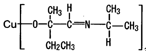
Compound No.24
