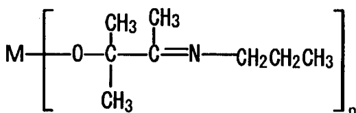
Compound No.13
