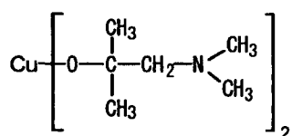
Comparative Compound 1
