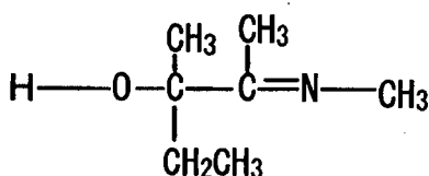
Compound No.75
