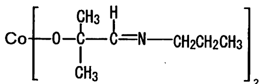
Compound No.53
