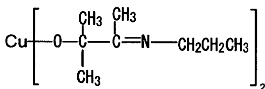
Compound No.29
