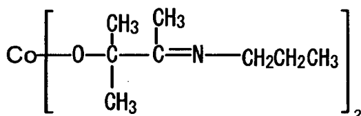
Compound No.61
