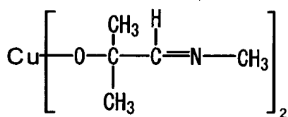
Compound No.17
