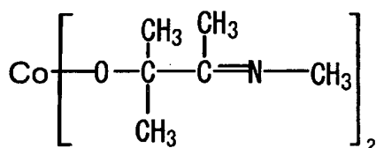
Compound No.57
