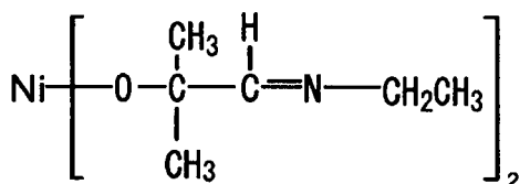
Compound No.35
