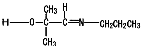
Compound No.69
