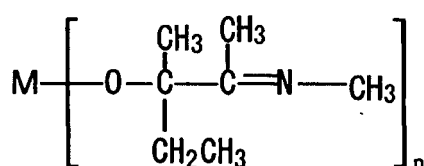
Compound No.10
