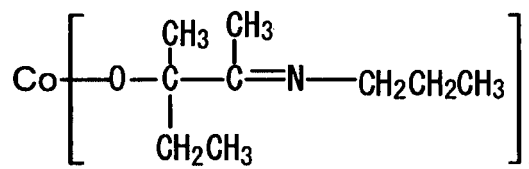
Compound No.62
