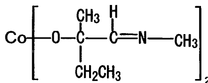
Compound No.50
