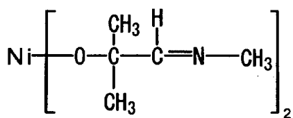
Compound No.33
