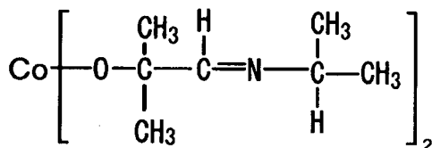
Compound No.55
