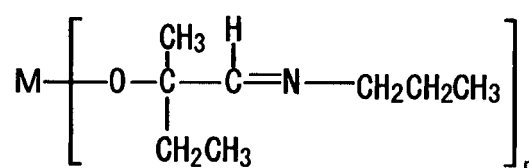
Compound No.6
