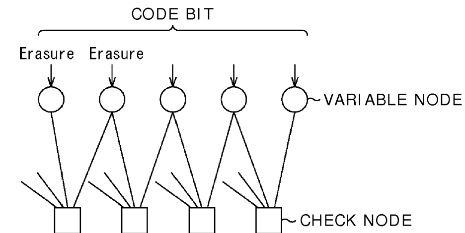
STAIRCASE STRUCTURE PORTION OF Tanner Graph
