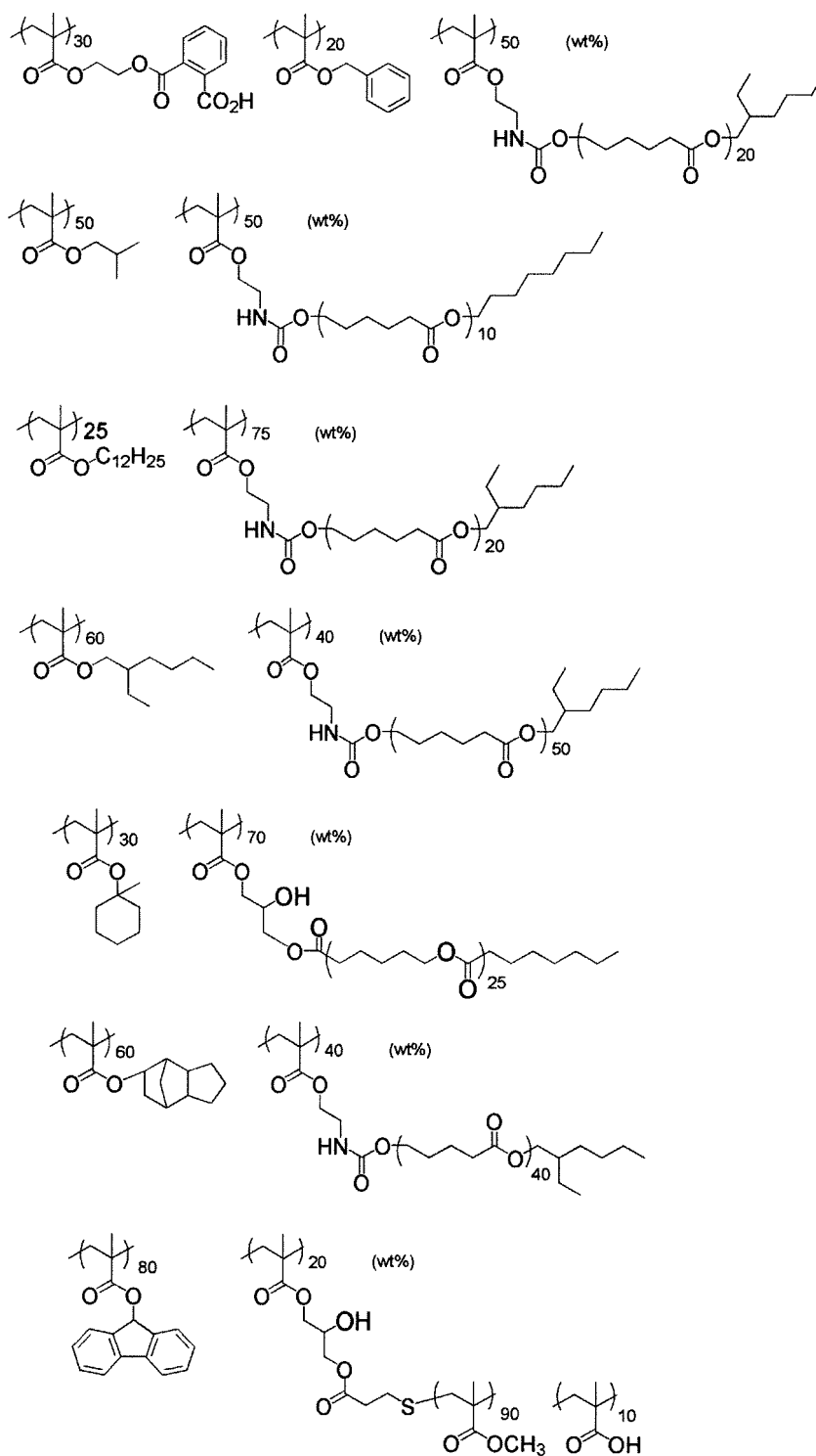
[Chemical formula 9]
