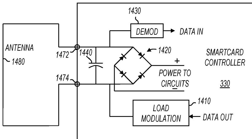
FIG. 14 (PRIOR ART)
