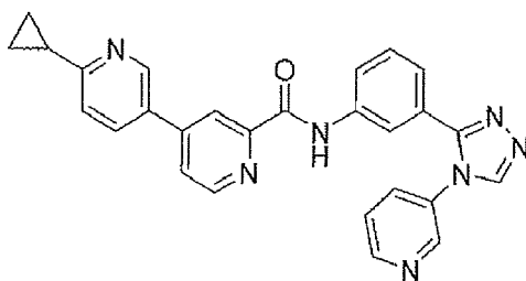
6-cyclopropyl-N-(3-(4-(pyridin-3-yl)-4H-1,2,4-triazol-3-yl)phenyl)-3,4'-bipyridine-2'-carboxamide;
