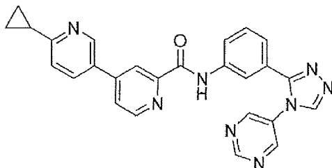
6-cyclopropyl-N-(3-(4-(pyrimidin-5-yl)-4H-1,2,4-triazol-3-yl)phenyl)-3,4-bipyridine-2'-carboxamide;
