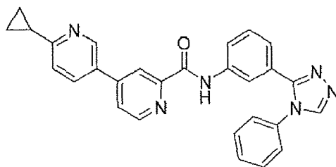
6-cyclopropyl-N-(3-(4-phenyl-4H-1,2,4-triazol-3-yl)phenyl)-3,4'-bipyridine-2-carboxamide;
