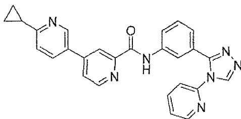
6-cyclopropyl-N-(3-(4-(pyridin-2-yl)-4H-1,2,4-triazol-3-yl)phenyl)-3,4'-bipyridine-2'-carboxamide;
