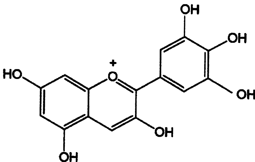
Chemical Formula (1)
