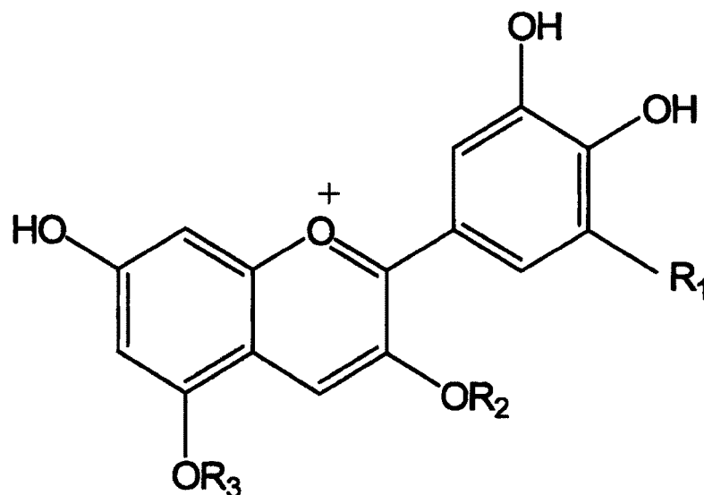
Chemical Formula (2)
