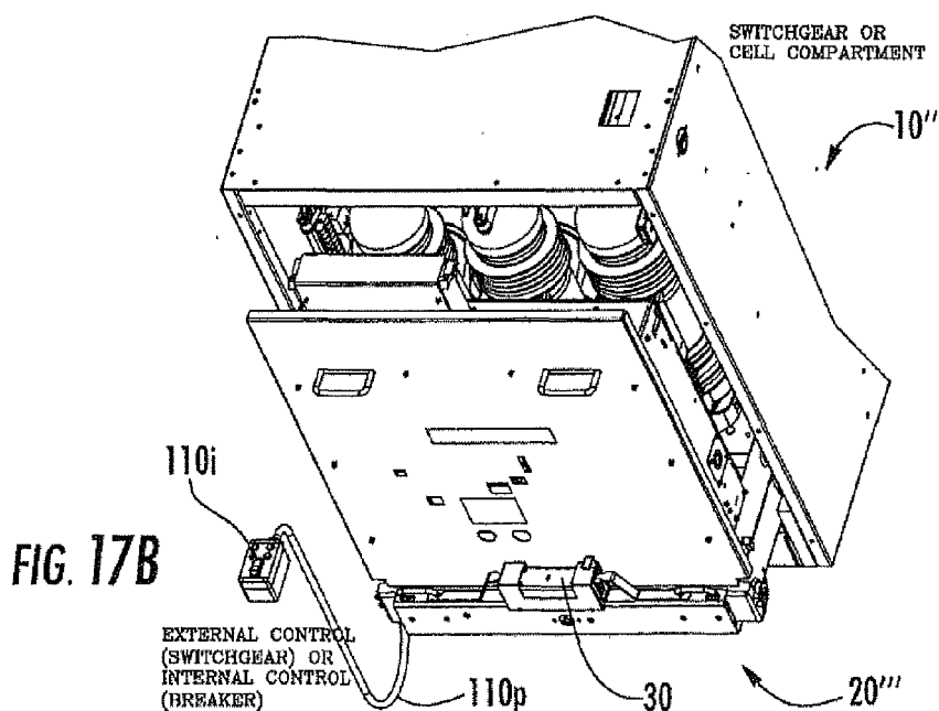
THE CRADLE ASSIST KIT INSTALLED, EXTERNALLY OR INTEGRATED WITH CRADLE OR BREAKER ITSELF, CAN ALSO BE POWERED BY EXTERNAL OR REMOTE CONTROL (E.G. CONTROL CONNECTED TO BREAKER OR SWITCHGEAR VIA UMBILICAL CORD)
