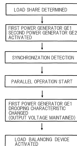
FLOW OF SHIFT TO PARALLEL OPERATION
