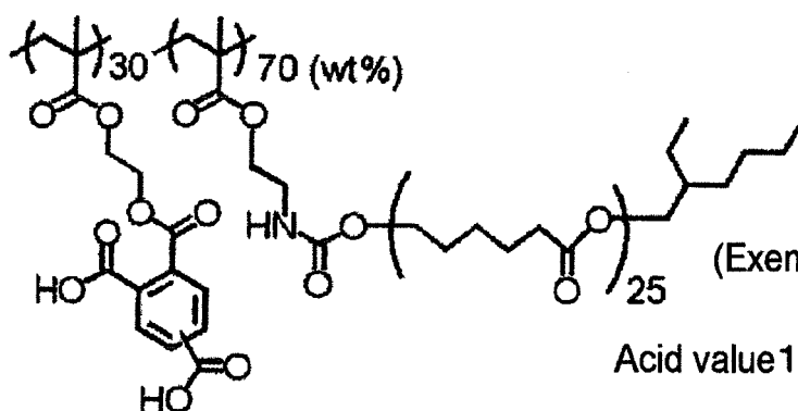
(Exemplary Compound 17) Acid value 154mgKOH/g
