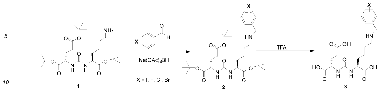
Scheme A. General pathway for the synthesis of halogenated Glu-Urea-Lys(N-benzyl-X) analogs (3).
