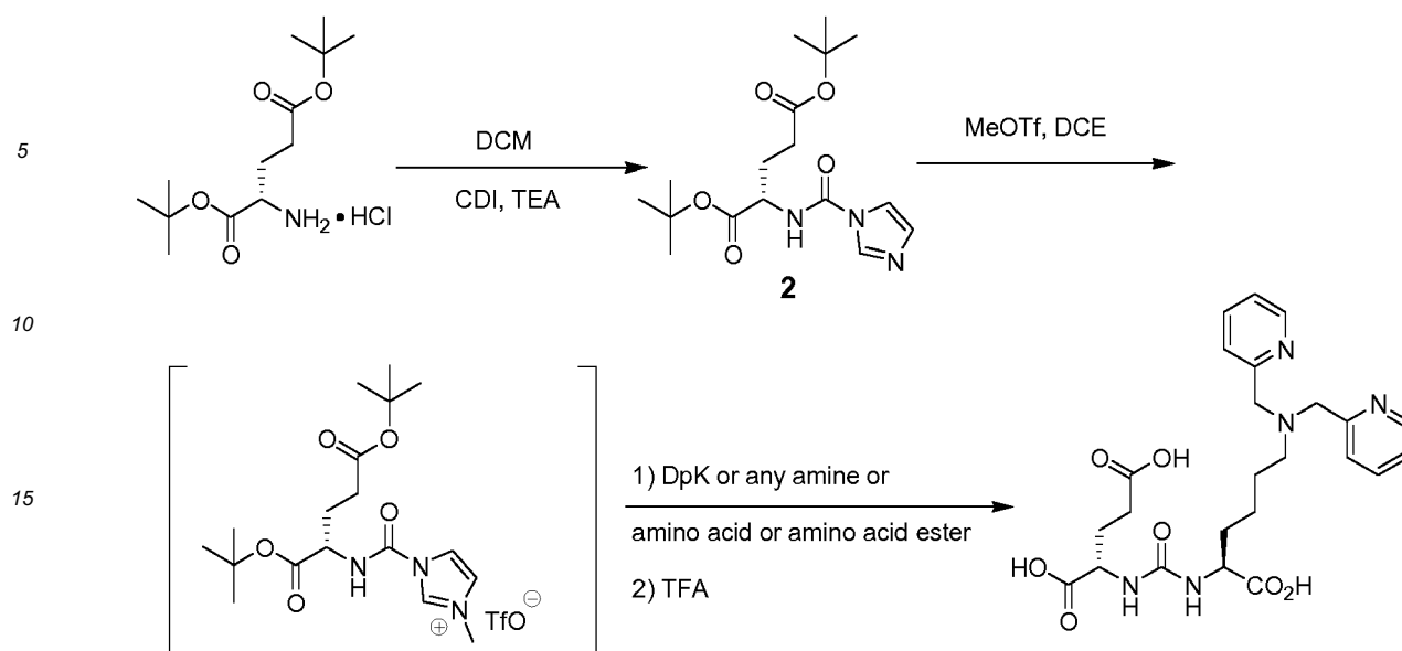
Scheme 1. General pathway for the synthesis of PSMA compounds.
