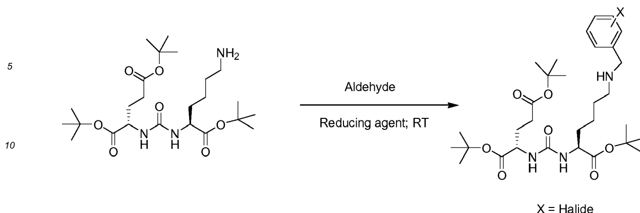
Scheme 3. General pathway for the synthesis of halogenated PSMA compounds.
