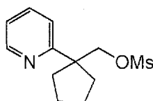
Methanesulfonic acid 1-pyridin-2-yl-cyclopentylmethyl ester
