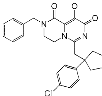
2-benzyl-6-((1-(4-chlorophenyl)cyclopentyl)methyl)-9-hydroxy-3,4-dihydro-1H-pyrazino[1,2-c]pyrimidine-1,8(2H)-dione
