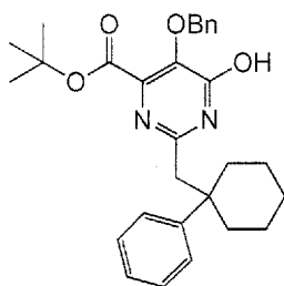
5-Benzyloxy-6-hydroxy-2-(1-phenyl-cyclohexylmethyl)-pyrimidine-4-carboxylic acid tert-butyl ester
