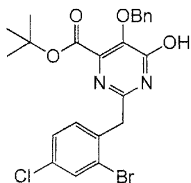
5-Benzyloxy-2-(2-bromo-4-chlorobenzyl)-6-hydroxy-pyrimidine-4-carboxylic acid tert-butyl ester
