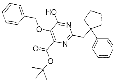
5-Benzyloxy-6-hydroxy-2-(1-phenyl-cyclopentylmethyl)-pyrimidine-4-carboxylic acid tert-butyl ester
