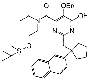
5-Benzyloxy-6-hydroxy-2-(1-naphthalen-2-yl-cyclopentylmethyl)-pyrimidine-4-carboxylic acid [2-(tert-butyl-dimethyl-silanyloxy)-ethyl]-isopropyl-amide
