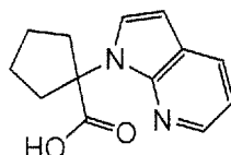
1-Pyrrolo[2,3-b]pyridin-1-yl-cyclopentanecarboxylic acid
