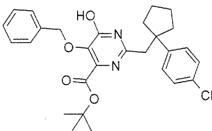
5-Benzyloxy-2-[1-(4-chloro-phenyl)-cyclopentylmethyl]-6-hydroxy-pyrimidine-4-carboxylic acid tert-butyl ester
