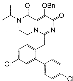
9-Benzyloxy-6-(5,4'-dichloro-biphenyl-2-ylmethyl)-2-isopropyl-3,4-dihydro-2H-pyrazino[1,2-c]pyrimidine-1,8-dione
