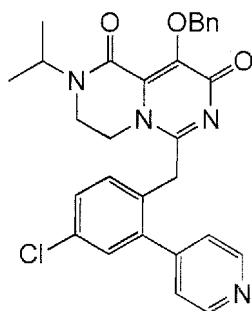
6-(4-Chloro-2-pyridin-4-yl-benzyl)-9-hydroxy-2-isopropyl-3,4-dihydro-2H-pyrazino[1,2-c]pyrimidine-1,8-dione
