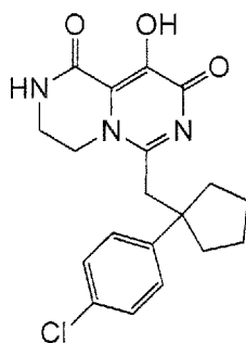
6-((1-(4-chlorophenyl)cyclopentyl)methyl)-9-hydroxy-3,4-dihydro-1H-pyrazino[1,2-c]pyrimidine-1,8(2H)-dione
