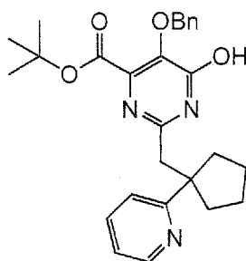
5-Benzyloxy-6-hydroxy-2-(1-pyridin-2-yl-cyclopentylmethyl)-pyrimidine-4-carboxylic acid tert-butyl ester
