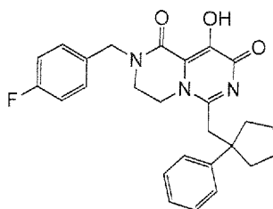
2-(4-Fluoro-benzyl)-9-hydroxy-6-(1-phenyl-cyclopentylmethyl)-3,4-dihydro-2H-pyrazino[1,2-c]pyrimidine-1,8-dione
