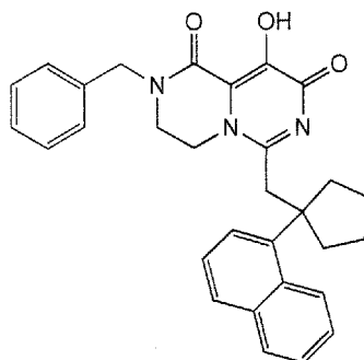
2-Benzyl-9-hydroxy-6-(1-naphthalen-1-yl-cyclopentylmethyl)-3,4-dihydro-2H-pyrazino[1,2-c]pyrimidine-1,8-dione
