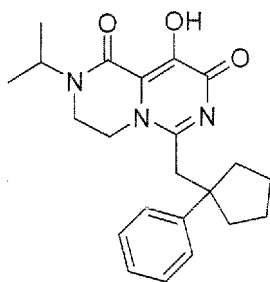
9-Hydroxy-2-isopropyl-6-(1-phenyl-cyclopentylmethyl)-3,4-dihydro-2H-pyrazino[1,2-c]pyrimidine-1,8-dione
