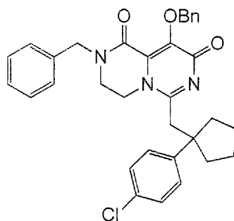
2-benzyl-9-(benzyloxy)-6-((1-(4-chlorophenyl)cyclopentyl)methyl)-3,4-dihydro-1H-pyrazino[1,2-c]pyrimidine-1,8(2H)-dione
