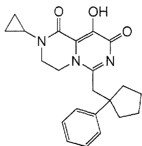
2-Cyclopropyl-9-hydroxy-6-(1-phenyl-cyclopentylmethyl)-3,4-dihydro-2H-pyrazino[1,2-c]pyrimidine-1,8-dione
