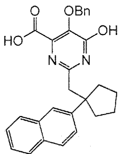
5-Benzyloxy-6-hydroxy-2-(1-naphthalen-2-yl-cyclopentylmethyl)-pyrimidine-4-carboxylic acid
