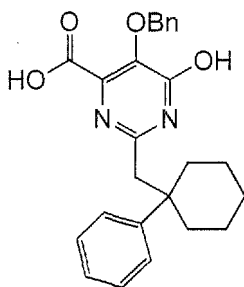
5-Benzyloxy-6-hydroxy-2-(1-phenyl-cyclohexylmethyl)-pyrimidine-4-carboxylic acid
