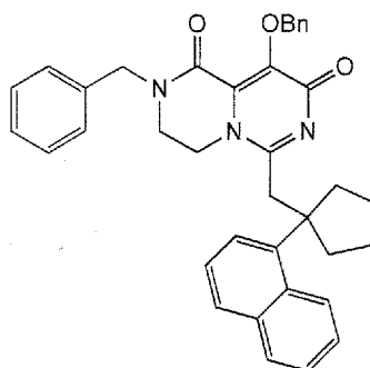
2-Benzyl-9-benzyloxy-6-(1-naphthalen-1-yl-cyclopentylmethyl)-3,4-dihydro-2H-pyrazino[1,2-c]pyrimidine-1,8-dione
