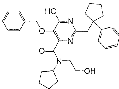
5-Benzyloxy-6-hydroxy-2-(1-phenyl-cyclopentylmethyl)-pyrimidine-4-carboxylic acid cyclopentyl-(2-hydroxyethyl)-amide
