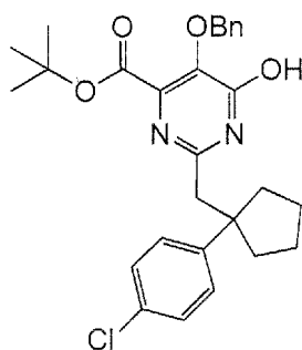
5-Benzyloxy-2-[1-(4-chloro-phenyl)-cyclopentylmethyl]-6-hydroxy-pyrimidine-4-carboxylic acid tert-butyl ester
