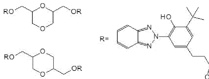
FORMULA II
