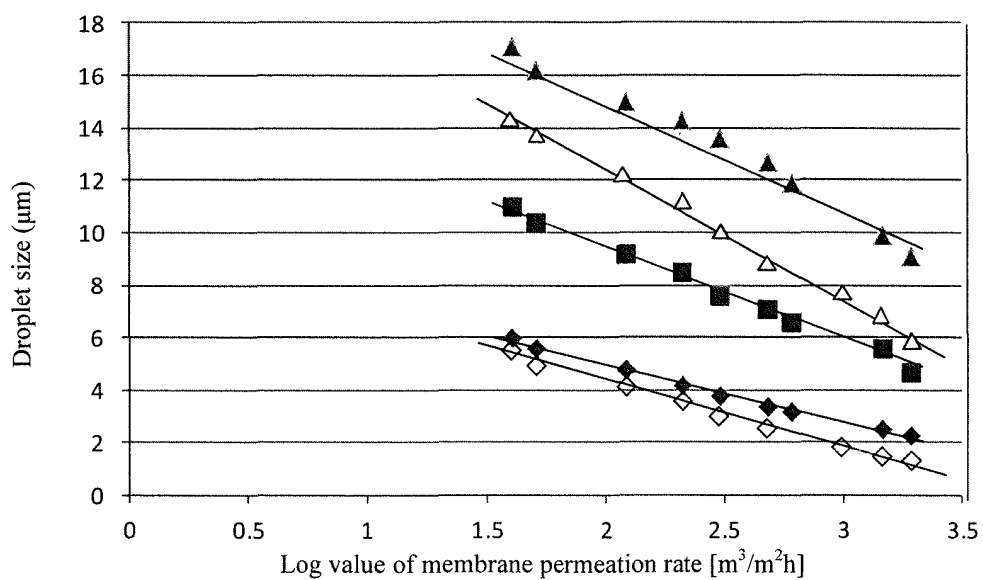
FIG Influence of membrane permeation rate on droplet size
