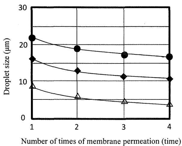
FIG. 8 Relationship of the viscosities of continuous phase liquid and disperse phase liquid with droplet size (B) ●; 1 mPa·s, ◆; 55 mPa·s, △; 85 mPa·s Disperse phase viscosity; 250 mPa·s
