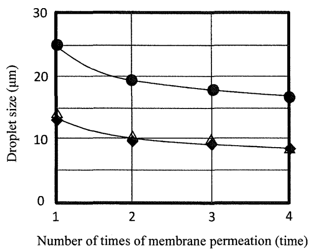
FIG. 7 Relationship of the viscosities of continuous phase liquid and disperse phase liquid with droplet size (A) ●; 1 mPa·s, ◆; 55 mPa·s, △; 85 mPa·s Disperse phase viscosity; 17 mPa·s
