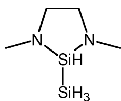
1,1-(N,N'- dimethylethylenediamino)disil ane
