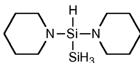
1,1-dipiperidinodisilane
