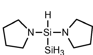
1,1-dipyrrolidinodisilane
