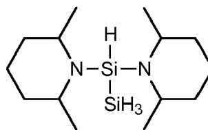
1,1-di(2,6-dimethylpiperidino)disilane
