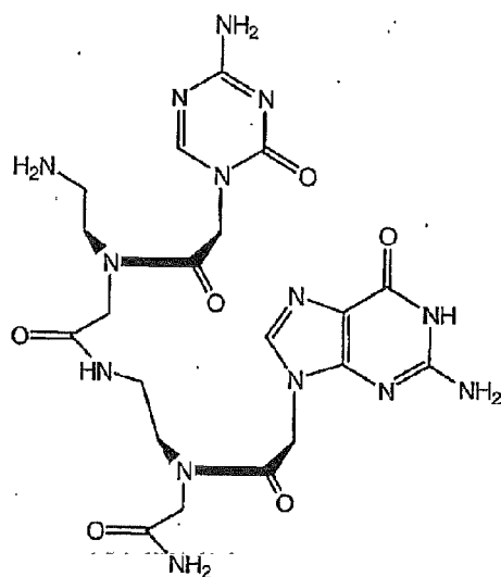
-DpnaG- Islet with Peptide Backbone
