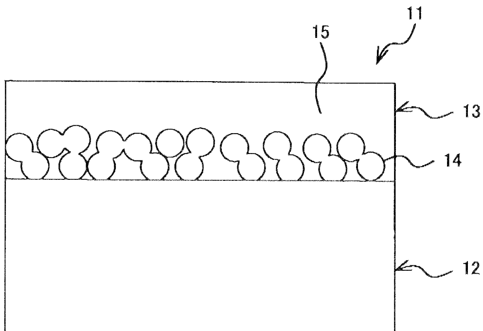
FIG. 10 PRIOR ART
