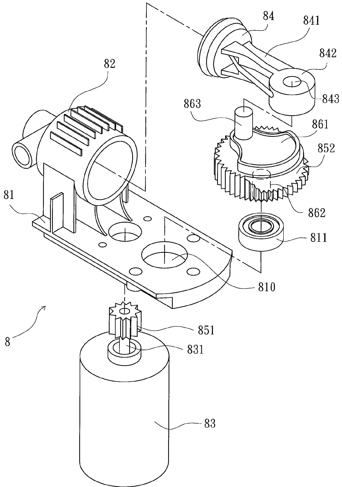
FIG. 6 Prior Art
