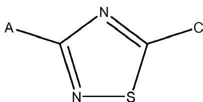
Formula VI
