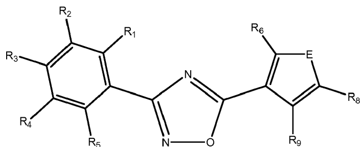
Formula IVb
