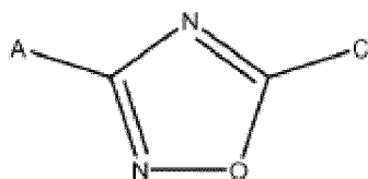
Formula IV
