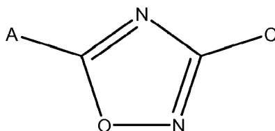
Formula V
