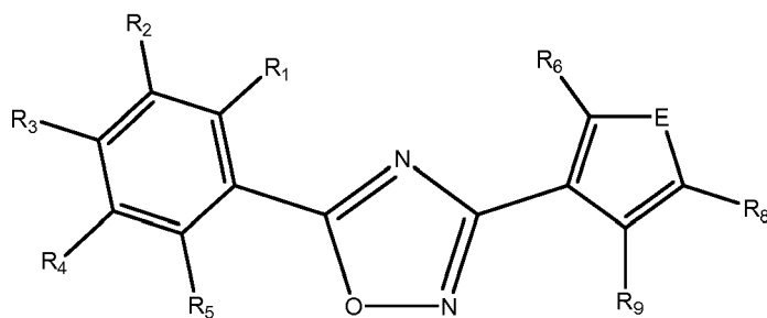
Formula Vb
