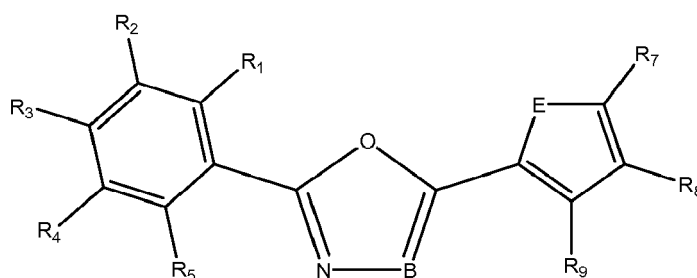
Formula IIa
