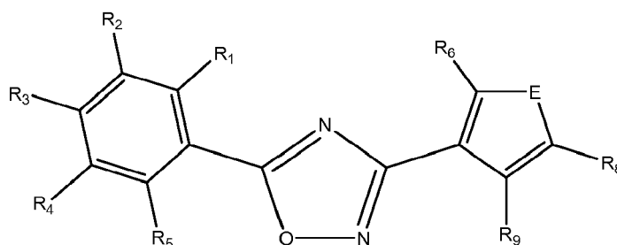
Formula Vb
