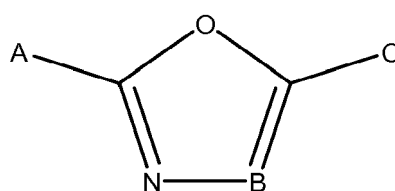
Formula II
