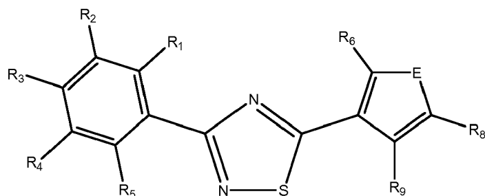
Formula VIb
