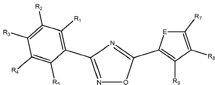
Formula IVa
