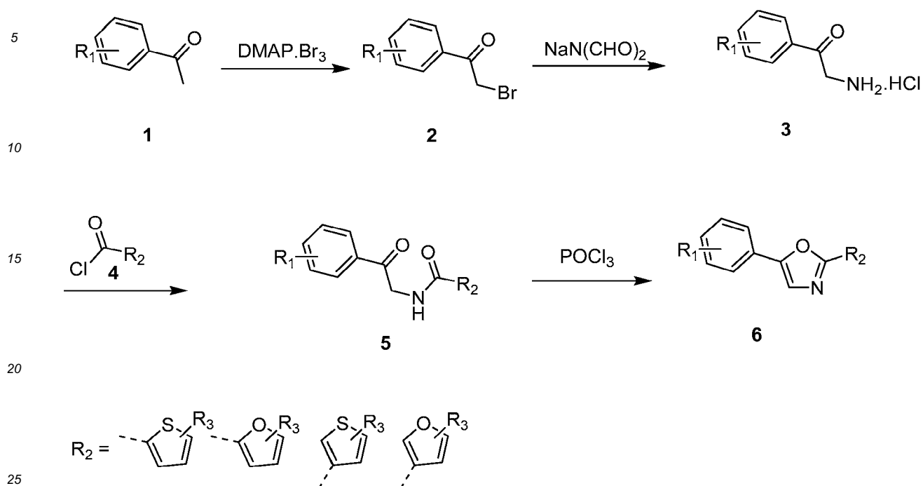
Scheme 1: Synthetic scheme to compounds of the Formula Ia and Ib
