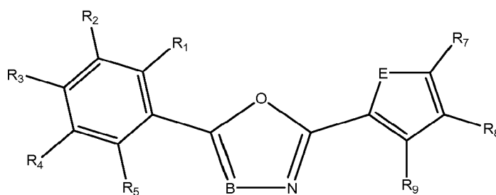
Formula Ia
