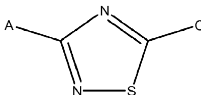
Formula VI
