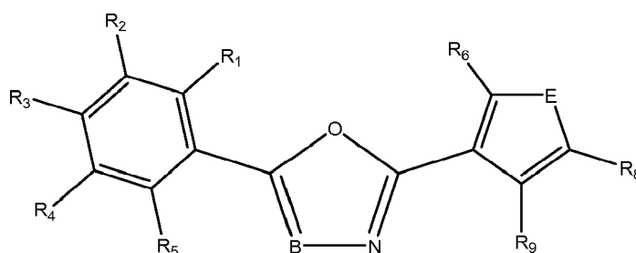
Formula Ib
