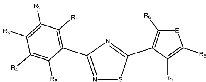
Formula VIb
