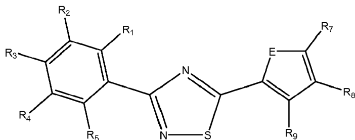
Formula VIa
