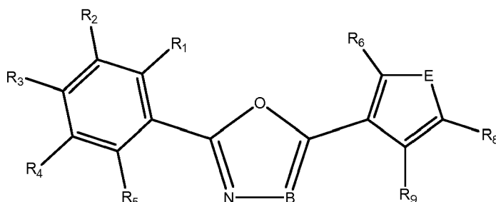
Formula IIb
