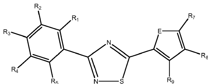
Formula VIa
