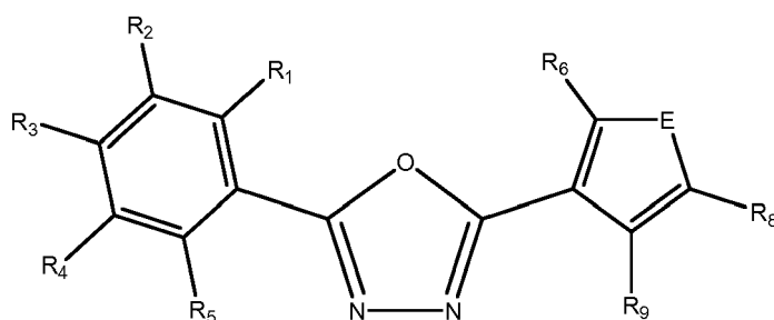
Formula IIIb
