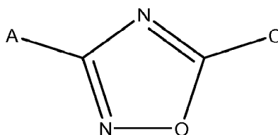
Formula IV
