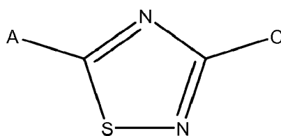
Formula VII
