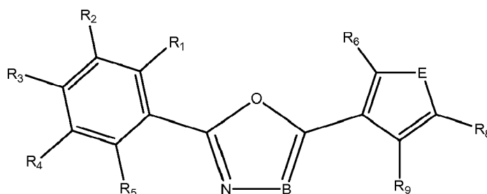
Formula IIb
