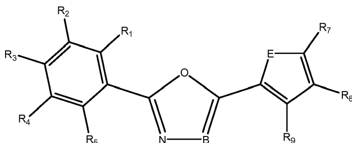
Formula IIa
