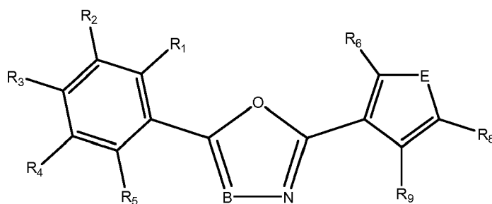
Formula Ib
