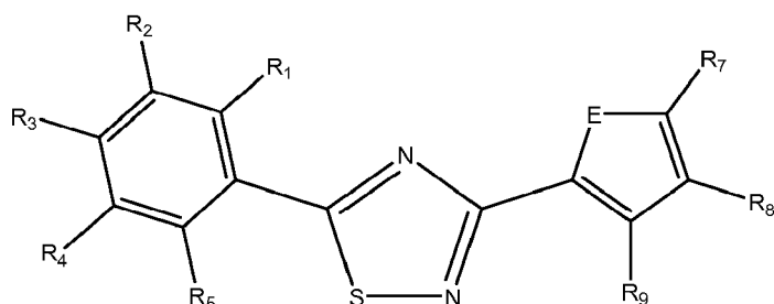
Formula VIIa
