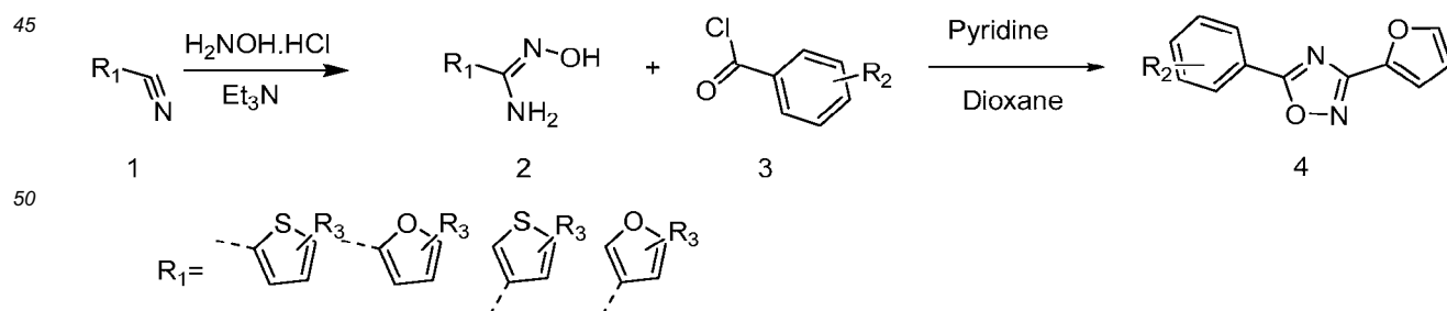
Scheme 5: Synthetic scheme to compounds of the Formula Va and Vb
