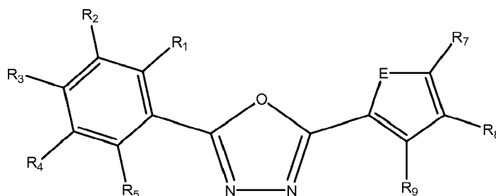
Formula IIIa
