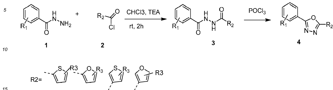
Scheme 3: Synthetic scheme to compounds of the Formula IIIa and IIIb
