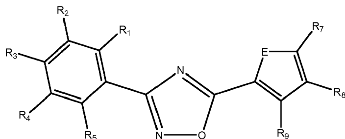
Formula IVa
