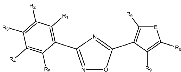
Formula IVb
