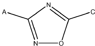
Formula IV
