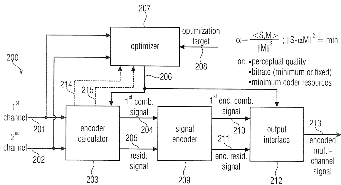
FIGURE 2 (AUDIO ENCODER)
