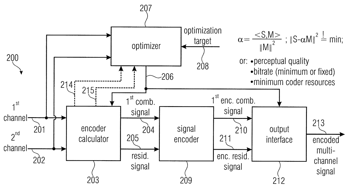
FIGURE 2 (AUDIO ENCODER)
