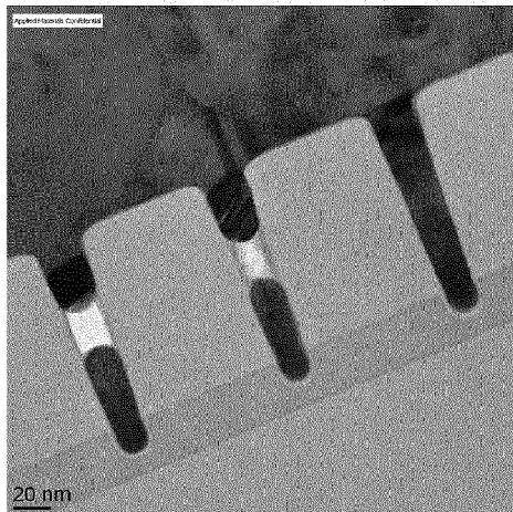
FIG. 10 (PRIOR ART)
